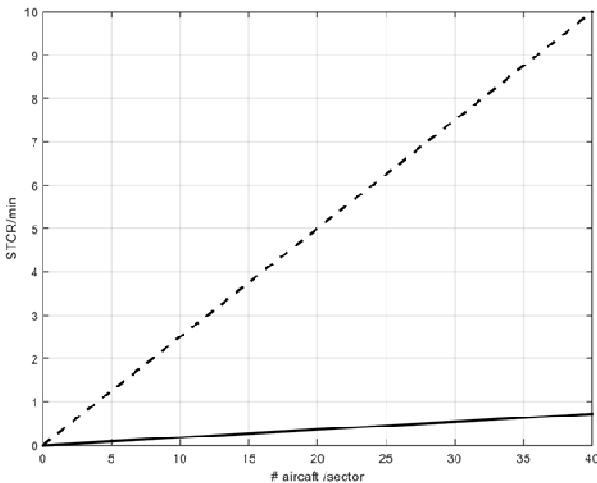
Figure 8. Predicted STCR activity frequency of an ATCo in the direct loop as a function of the hypothetical number of aircraft under iA3G model and traffic density considered. Solid curve: 3x 2005 high, no wind error; dashed curve: 3x 2005 high, 30 m/s wind prediction error.
