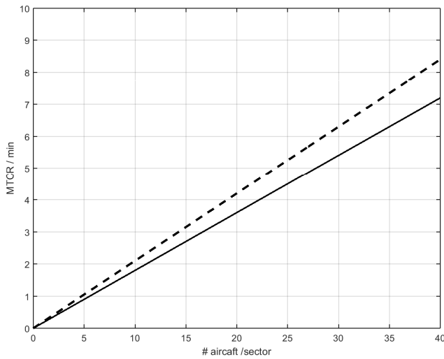
Figure 7. Predicted MTCR activity frequency of an ATCo as a function of the hypothetical number of aircraft to be controlled under the iA3G model and traffic density considered. Solid curve: 3x 2005 high, no wind error; dashed curve: 3x 2005 high, 30 m/s wind prediction error.
