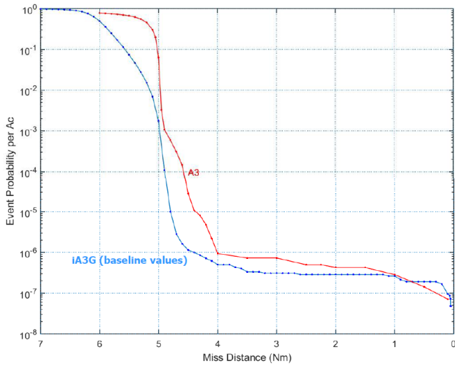
Figure 3. Estimated miss event probability per aircraft in the 8-a/c encounter scenario, as function of horizontal miss distance for the iA3G model vs. the A3 model. Source [14].
