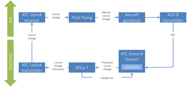
Figure 2. Information flow in the tactical layer of iA3G ConOps; STCR-IIS is part of the ATC ground system.
