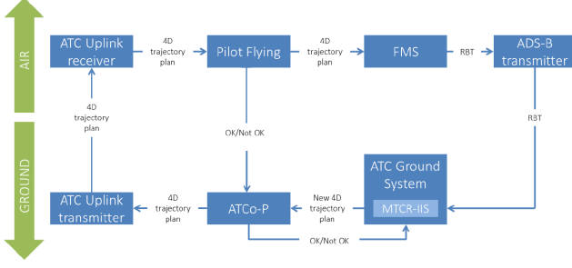
Figure 1. 4D trajectory plan information flow in TBO layer of iA3G ConOps; MTCR-IIS is part of the ATC ground system.
