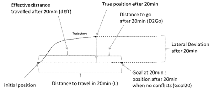
Figure 9. Flight efficiency measures.
