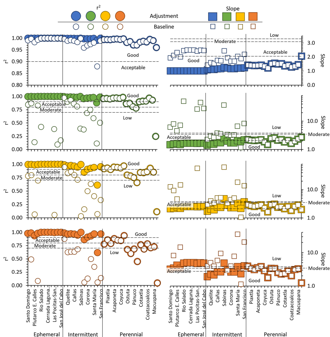
Figure 6. Performance assessment of the baseline and the new (adjustment) reference values of the frequency factors of occurrence per environmental objective class (A = blue, B = green, C = yellow, and D = orange) for environmental water allocation in ephemeral streams, intermittent, and perennial rivers. Coefficients of determination ( r^2 ) on the left panel (circles, white baseline, and colored adjustment), and slope values on the right panel (squares, white baseline, and colored adjustment; environmental objective classes B, C, and D displayed at a logarithmic scale). Thresholds for the performance classes displayed dashed lines.
