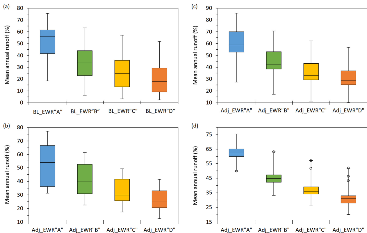
Figure 5. Central and full range of environmental water reserve volumes (EWR in percentage of the mean annual runoff) per environmental objective class (A = blue, B = green, C = yellow, and D = orange). (a) The method baseline (BL) criteria applied in the 40 basins, and the adjustments (Adj) based on the new criteria of frequency of occurrence reference values for (b) ephemeral ( n = 11 ), (c) intermittent ( n = 12 ), and (d) perennial rivers ( n = 17 ; outliers displayed in circles).
