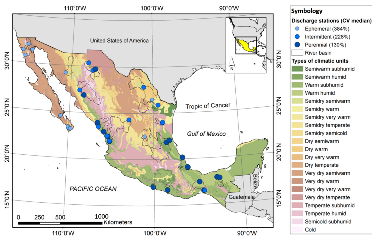
Figure A2. Location of study basins, flow type at the gauged point, the median of the coefficient of variation (CV), and types of climates based on the Köppen climatic classification system.
