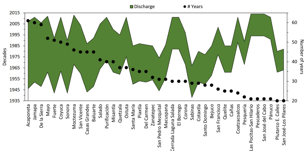
Figure 2. Periods of streamflow analysis of the river sites. Decades comprised in the left vertical axis (colored area), while the number of consecutive years in the right vertical axis (dots).
