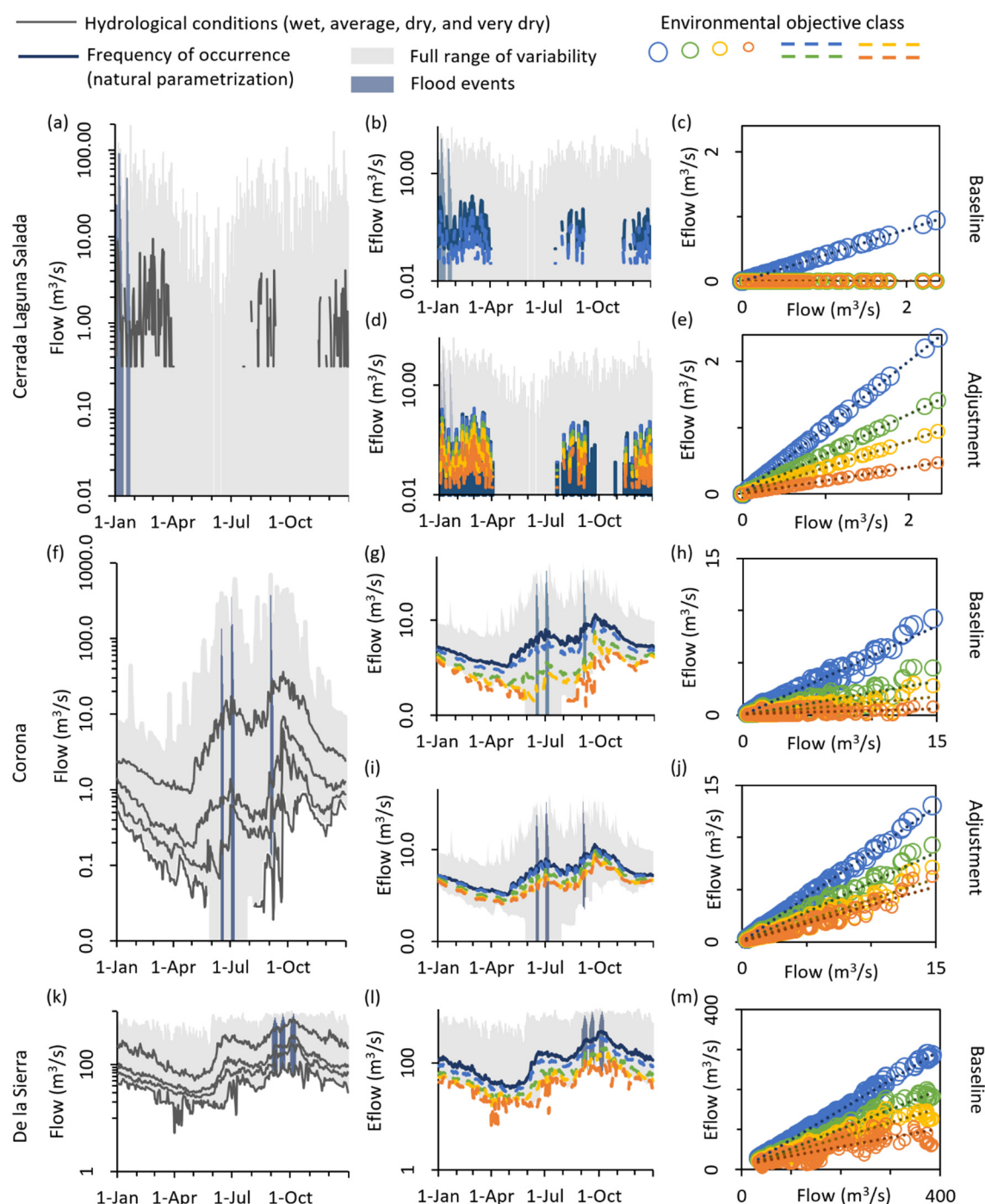
Figure 3. Performance assessment of the new frequency factors of occurrence for environmental flow allocation at three illustrative river sites, Cerrada Laguna Salada ephemeral stream, Corona intermittent river, and De la Sierra perennial river. First, wet, average, dry, and very dry conditions were computed at a daily scale for each calendar hydrological year based on each river site's complete set of flow records (hydrographs on the left; (a,f,k) panels; flow rate displayed at a logarithmic scale). Second, integrated environmental flows were obtained based on the reference factors (values) for both the baseline and the adjustment (Table 1) according to the environmental objective classes (Equation (5)). The regime representative of the hydrological conditions was also calculated and plotted based on the corresponding values for natural parametrization, that is to say, 25%, 50%, 15%, and 10% (hydrographs in the middle; ((b,d,g,i,l) panels). Third, the metrics for the performance assessment ( r^2 and slope values) were calculated based on the correlation of the natural parametrization and the model outcomes per environmental objective (scatterplots on the right; ((c,e,h,j,m) panels). This procedure was repeated for all the study sites and critically examined for each subset and the full set of outcomes according to the performance criteria previously established.
