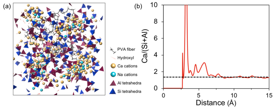
Fig. 7. (a) Snapshot of the in situ polymerization process of C-(N)-A-S-H gel around a PVA molecule in a simulation box with an average Ca/(Si+Al) of 1.3 and Al/Si ratio of 0.5. (b) Evolution of the Ca/(Si+Al) ratio as a function of the distance from the oxygen atoms of the PVA fibers. The black dashed indicates the average Ca/(Si+Al) ratio of 1.3.
