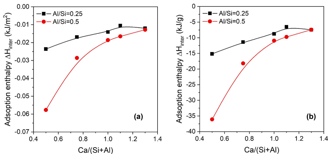
Fig. 12. Adsorption enthalpies in (a) \text{kJ/m}^2 and (b) \text{kJ/g} attributed to the hydrogen bonds between the PVA molecules and the C-(N)-A-S-H gel for the composites with Al/Si ratio of 0.25 (black squares) and 0.5 (red dots) at the considered theoretical \text{Ca}/(\text{Si}+\text{Al}) ratios.
