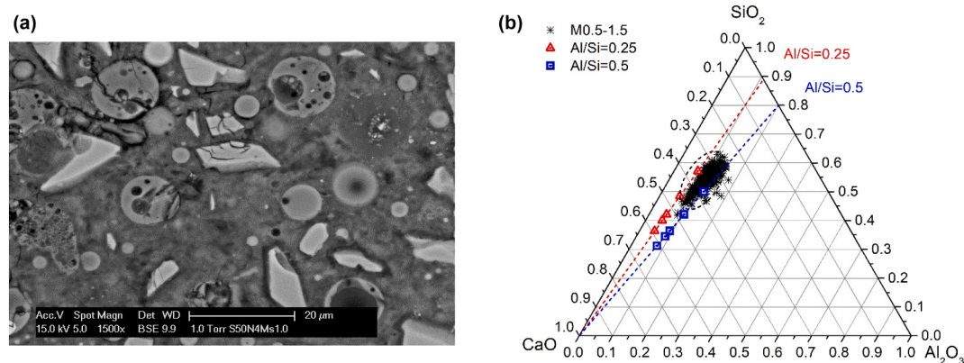
Fig. 13. (a) Representative BSE images of M1.0 AASF matrix and (b) ternary diagram of \text{CaO-SiO}_2\text{-Al}_2\text{O}_3 of EDX spot analysis for reaction product in the M0.5-M1.5 AASF matrices and C-(N)-A-S-H model for MD simulation (Al/Si = 0.25 and Al/Si = 0.5).
