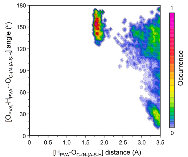
Fig. 10. Combine distribution function of hydrogen bond distances and angles between the PVA fibers and the C-(N)-A-S-H surfaces. Red colors correspond to the most probable configurations, while the blue ones are related to the less probable configurations.
