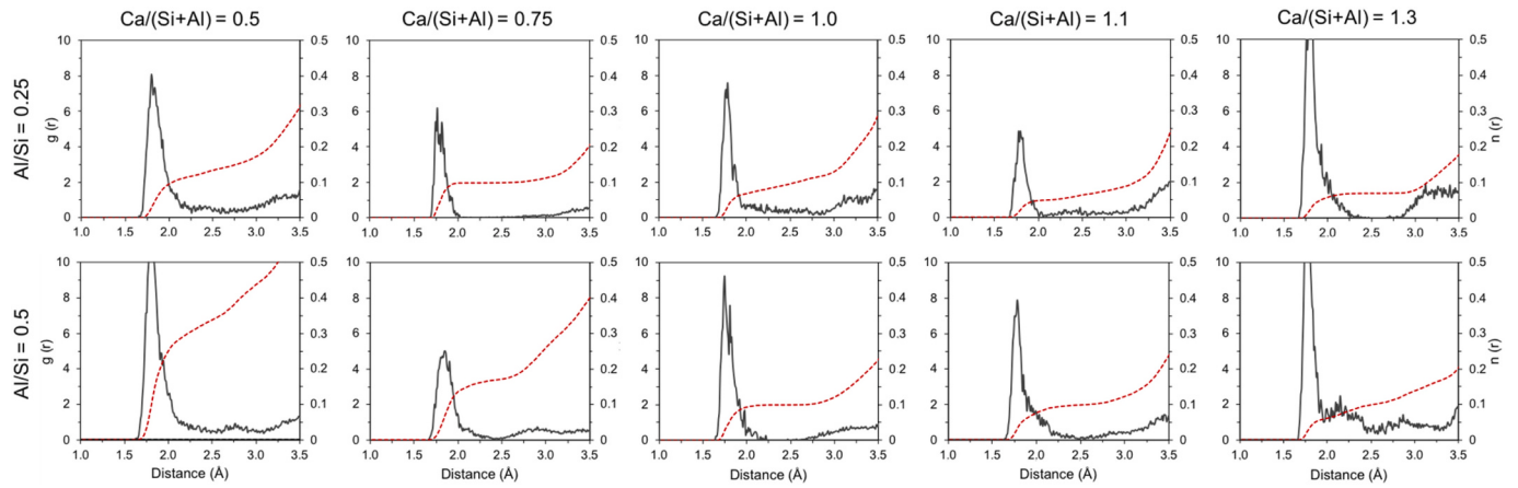
Fig. 8. Radial distribution functions (black continuous lines) and coordination numbers (red dashed lines) for H_{PVA}-O_{C-(N)-A-S-H} with Ca/(Si+Al) ratios of 0.5, 0.75, 1.0, 1.1 and 1.3 at Al/Si ratios of 0.25 and 0.5.
