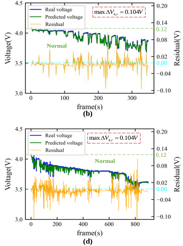
Fig. 17. The prediction result of vehicle No.4 from selected discharge segment (a) 1# and (c) 2# without outlier elimination; The prediction result from selected discharge segments (b) 1# and (d) 2# with outlier elimination utilizing boxplot.
