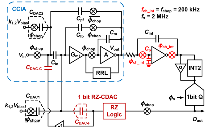
Fig. 3. Proposed CC-CTΣΔM.
