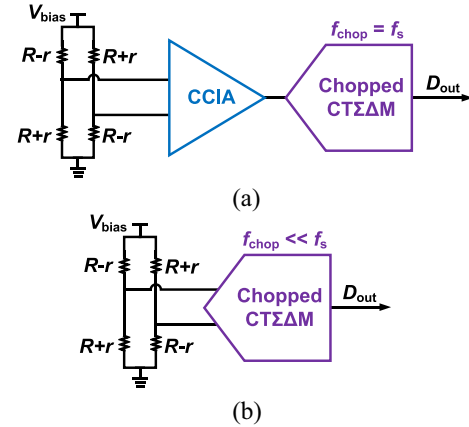
Fig. 1. Bridge readout with a (a) CCIA followed by a CT \Sigma\Delta M chopped at f_s and (b) stand-alone CT \Sigma\Delta M and f_{\text{chop}} \ll f_s .
