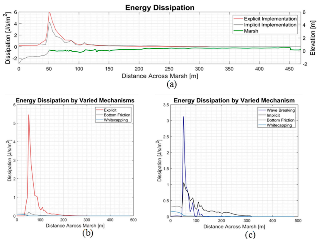
Figure 11. (a) Energy dissipation rates for the explicit (red) and implicit (gray) dissipation across the marshland shown in green. Panels (b) and (c) separate the dissipation rates by mechanism (bottom friction (gray), wave breaking (dark blue), whitecapping (light blue), implicit vegetation (black) and explicit vegetation (red)). The explicit representation is shown in panel (b) while the implicit representation is shown in panel (c).
