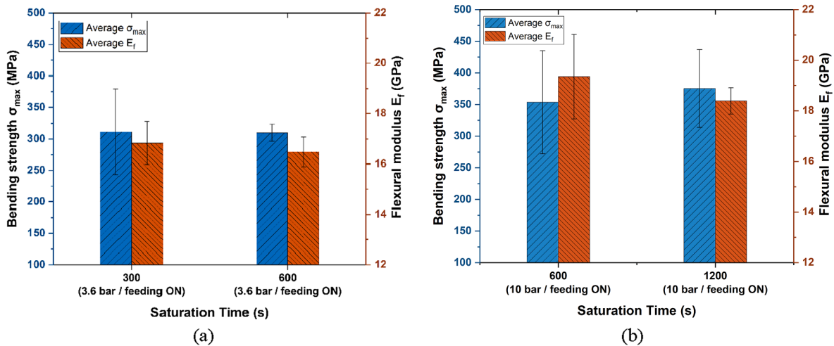
Fig. 11. Bending strength and bending modulus as a function of the saturation time; for saturation pressures of 3,6 bar (a) and 10 bar (b). ("feeding ON": resin injection was maintained during spacer collapse and polymer crystallization). (Injection at 240 °C).
