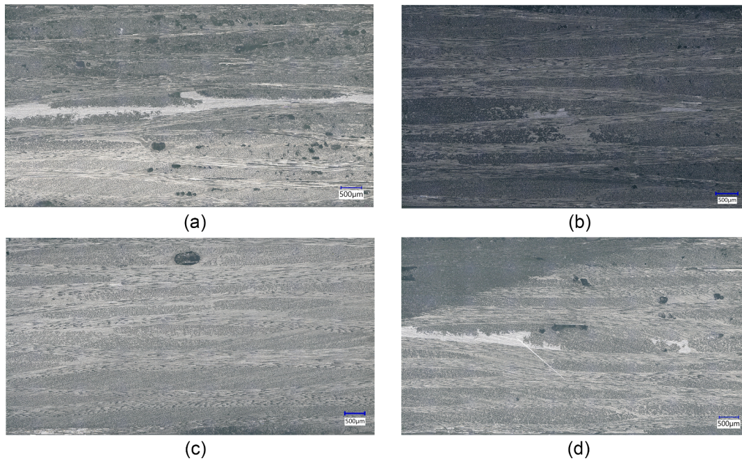
Fig. 17. Micrographs from samples cut close to the outlet on plates n°14 (a), 16 (b), 18 (c) and 23 (d).
