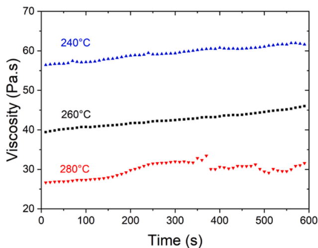
Fig. 1. Viscosity of HFP6 from shear-flow rheology measurements at 1 s -1 in air and at constant temperature.
