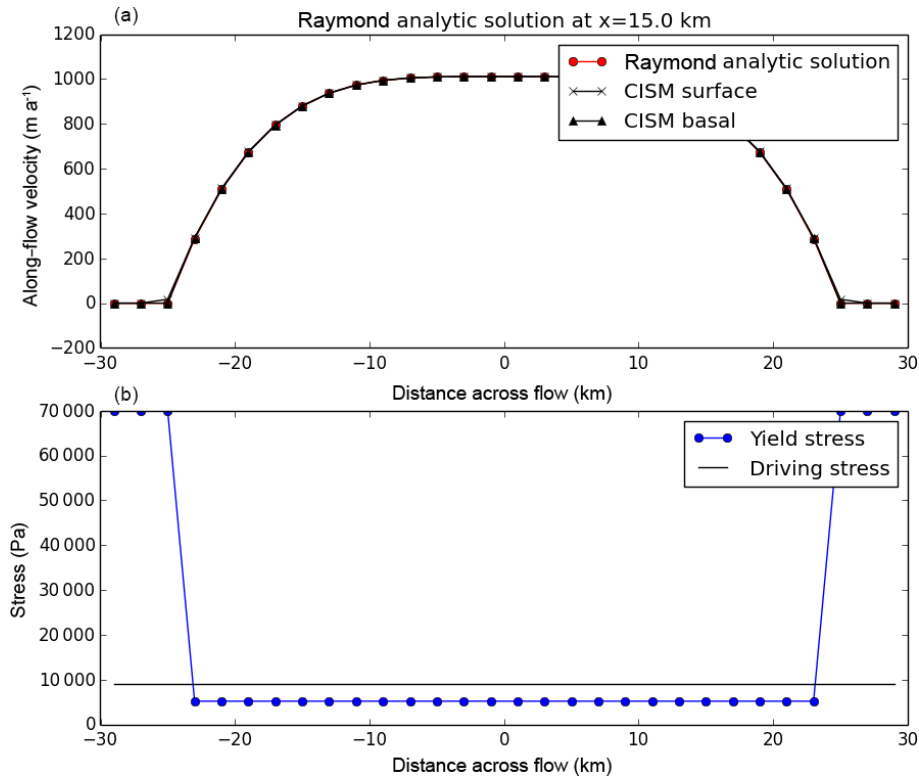
Figure 6. Results from the Raymond stream test using Glissade’s BP velocity solver. (a) Across-flow surface and basal velocity ( \text{m yr}^{-1} ) at x = 15 km compared to the analytic solution. At most points, the analytic and simulated solutions are indistinguishable. (b) Prescribed yield stress and gravitational driving stress (Pa).
