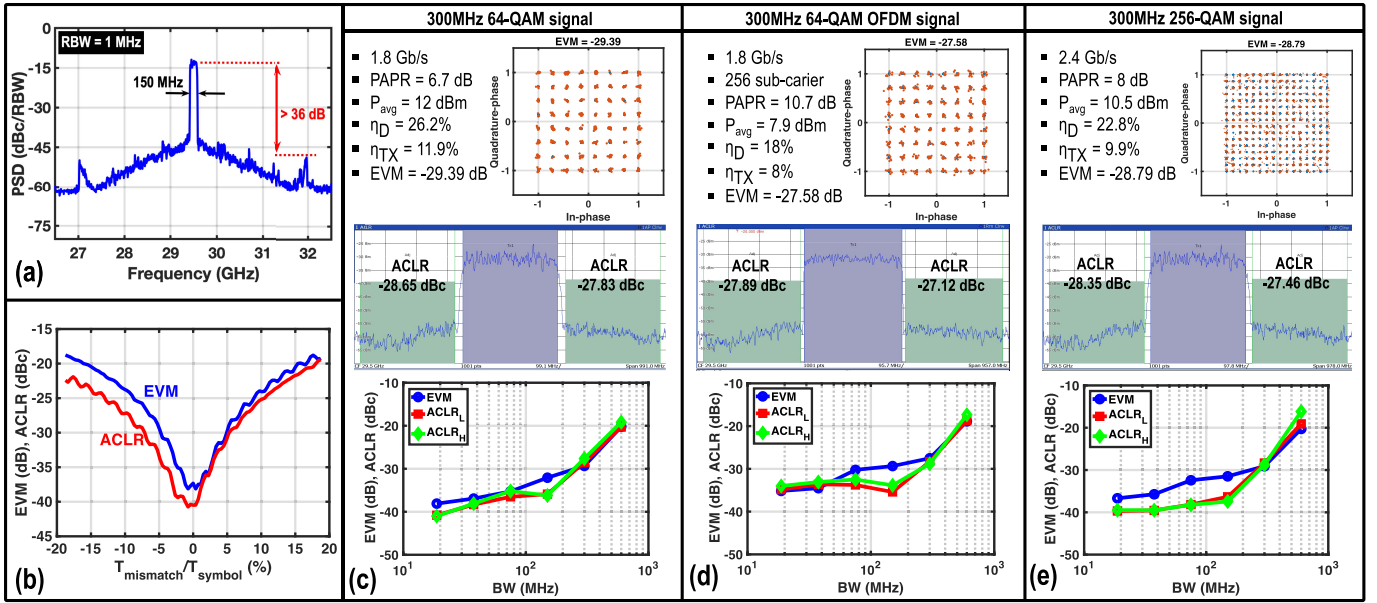
Fig. 18. Measured (a) output spectrum, and (b) EVM and ACLR versus delay mismatch between the AM and PM paths. Measured TX performance while transmitting a 300-MHz (c) 64-QAM single-carrier, (d) OFDM, and (e) 256-QAM single-carrier signal.
