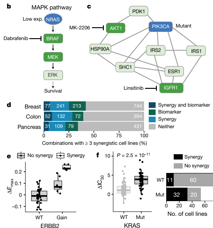
Fig. 3 | KRAS -mutant molecular context. d , Number of combinations with at least three synergistic cell lines and combination response biomarkers ( \Delta E_{max} or \Delta IC_{50} ). e , Gain of ERBB2 is associated with sapitinib + JQ1 combination response in breast and all synergistic cell lines have an ERBB2 amplification. f , KRAS mutation is associated with trametinib + MK-2206 combination response in a pan-tissue setting (left, two-sided Welch's t -test) and most synergistic cell lines harbour mutated KRAS (right). In box plots, the horizontal line shows the median, boxes extend across first and third quartiles, and whiskers extend to 1.5× interquartile range.
