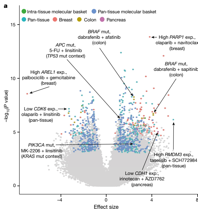
Fig. 3 | A biomarker pipeline incorporating multi-omics features identifies context-specific associations. a , Volcano plot of biomarkers associated with \Delta IC_{50} ( n = 2,006,328 ). Statistically significant large effect-size biomarkers ( n = 884 ) are coloured by analysis type. Examples discussed in the text and selected outliers are labelled. Exp., expression; mut., mutant. b , Schematic of MAPK pathway showing the relationship between NRAS and BRAF. Low expression of NRAS is a biomarker of certain dabrafenib-containing combinations. c , Network of interactors of PIK3CA, showing its position two nodes away from targets of MK-2206 and linsitinib. PIK3CA mutation is predictive of the linsitinib + MK-2206 combination response in the
