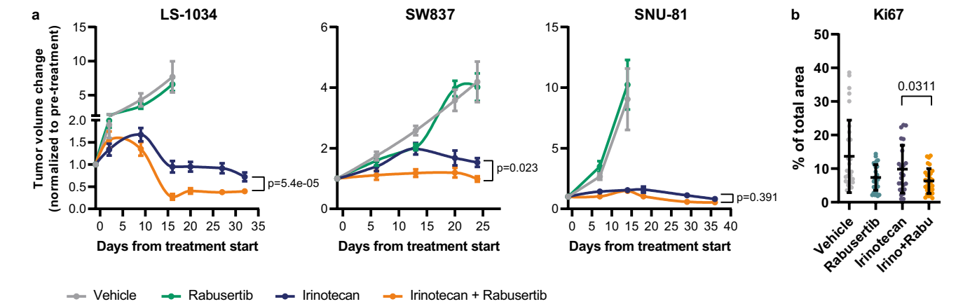
Extended Data Fig. 8 | In vivo validation of combined targeting of irinotecan and CHEK1 in colon cancer. a, Addition of rabusertib increases irinotecan response in two of three colon cancer xenograft models. NOD/scid mice were engrafted with colon cancer cell lines and treated with irinotecan (25 mg/kg twice a week) +/- rabusertib (200 mg/kg daily) for 24–35 days. Shown is average tumour volume change under treatment. LS-1034: n = 6 mice for vehicle, n = 11 for irinotecan, n = 12 for rabusertib and irinotecan+rabusertib. SW837: n = 6 mice for
