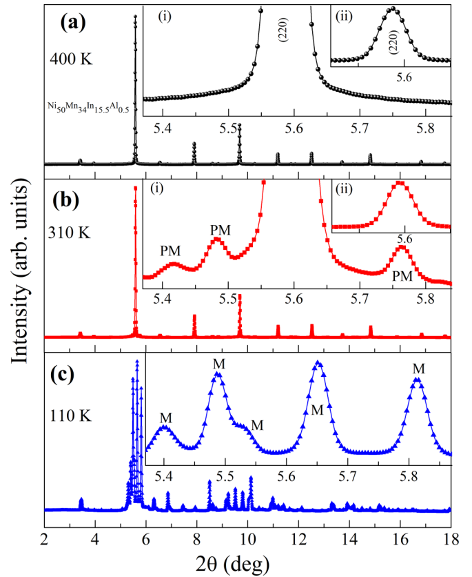
FIG. 2. Typical SXRPD patterns of \text{Ni}_{50}\text{Mn}_{34}\text{In}_{15.5}\text{Al}_{0.5} MSMA in the (a) austenite, (b) premartensite, and (c) martensite phases. An enlarged view around the most intense (220) Bragg peak for the austenite and the premartensite (PM) phases, given in inset (i) of (a) and (b), respectively, reveal the appearance of the satellite peaks [indicated by “PM” in the inset (i) of (b)] due to 3M like modulation in the PM phase. Untruncated view of the (220) cubic peak for the austenite and PM phases, given in inset (ii) of (a) and (b), respectively, reveal the absence of Bain distortion in the PM phase. The inset of (c) depicts the splitting of the most intense (220) cubic peak and appearance of the satellite peaks due to Bain distortion and 3M like modulation of the martensite (M) phase. The peaks related to the martensite phase are marked as “M” in the inset of (c).
