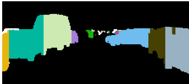
(e) Semantic stixels + Instances: Predicted offsets, GT assignment.
