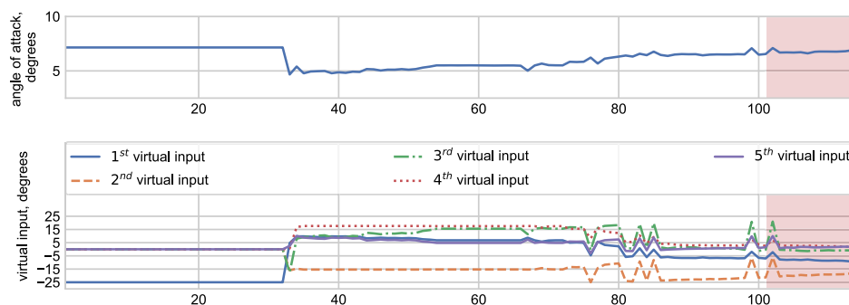
Fig. 14 Optimal inputs as calculated by the optimizer for a target lift coefficient of 0.75.
