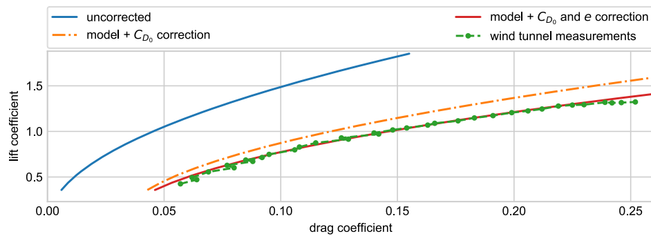
Fig. 6 Drag polar of the corrected aerodynamic model for a constant actuator angle of -22^\circ deg.
