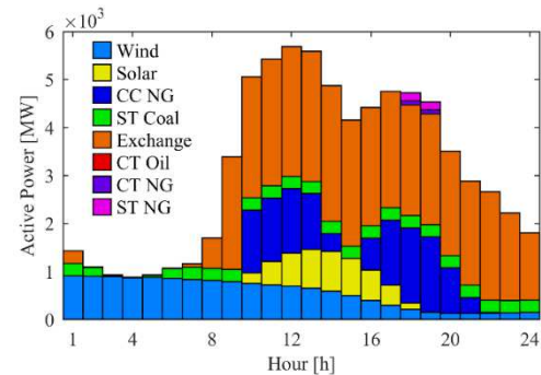
Fig. 3. Dispatched generation after the ZDAM solution.
