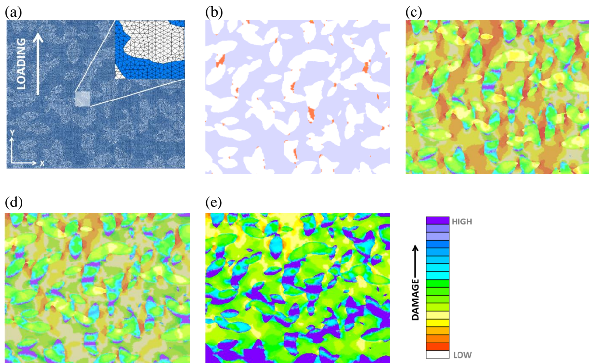
Figure 4: Finite element simulation of monotonic, displacement controlled loading with a strain rate of 0.02 \text{ s}^{-1} in y -direction. (a) Finite element mesh from processing 30 \times 30 \mu\text{m}^2 AFM phase image, for intermediate strain states of (b) 2%, (c), 4%, (d) 6% and (e) 10%.
