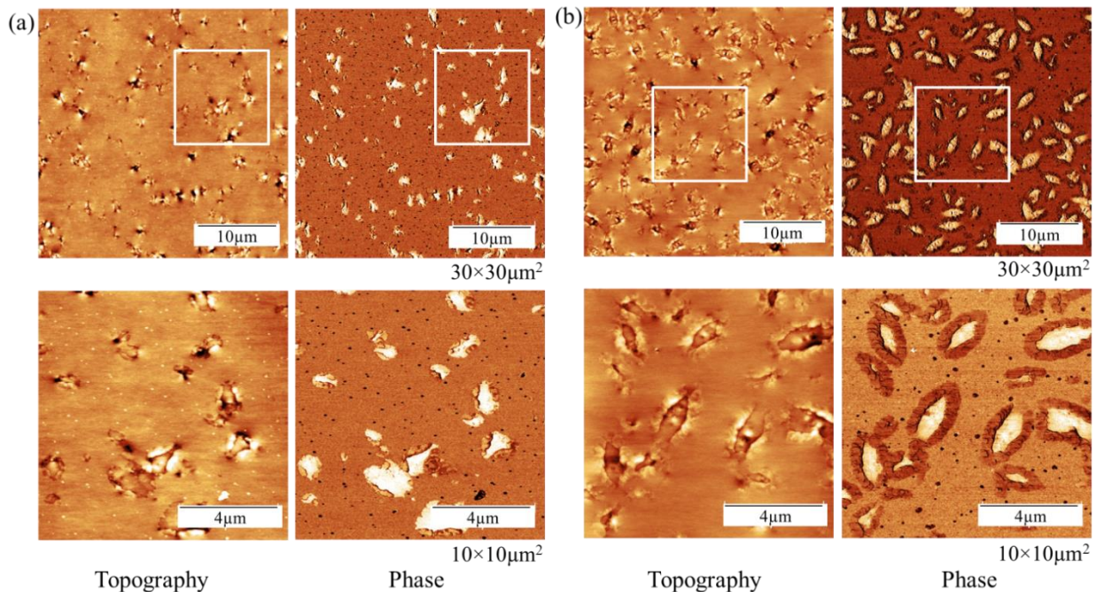
Figure 6: AFM topography and phase images of bitumen microstructure, captured at 25 °C after cooling from 90 °C to 25 °C. 30×30 μm 2 overview and 10×10 μm 2 zoomed in images of a) 70/100 and (b) 160/220.
