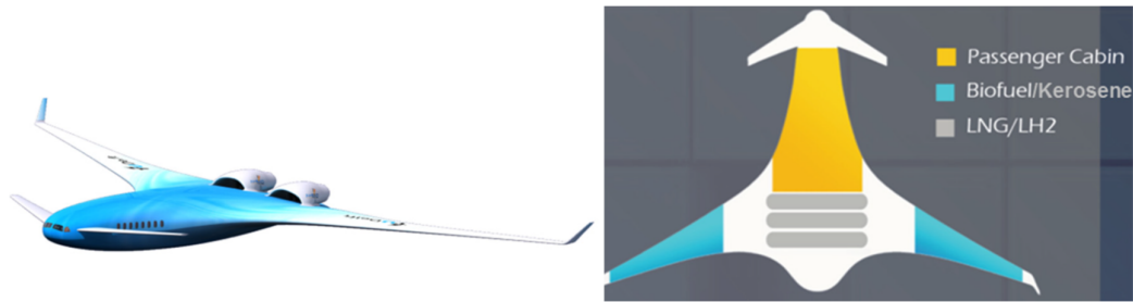
Figure 23. The multi-fuel blended-wing body investigated in the AHEAD project [37].
