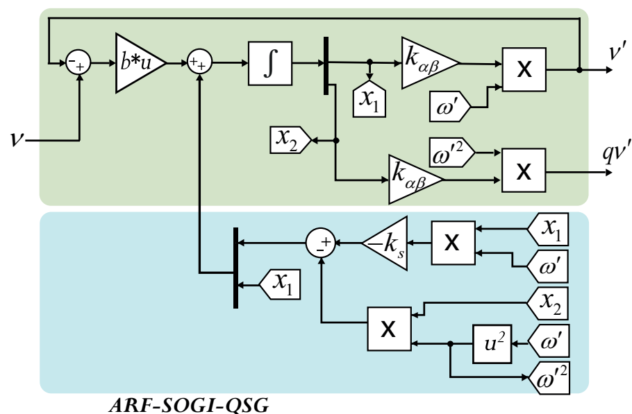
Figure 2. State space architecture of the ARF-SOGI-QSG.
