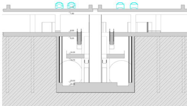
Station Section
