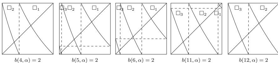
Fig. 12 Arrangements of T_{N,\alpha} with b = 2 ; in each case \alpha = \frac{\sqrt{2N+1}-1}{2}
