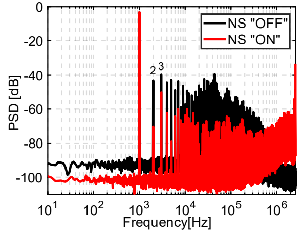
Fig. 7. Measured PSD of SAR ADC.
