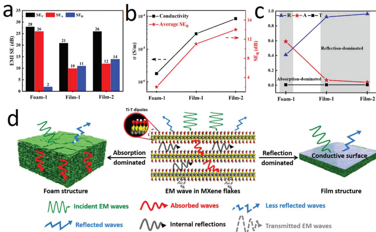
Figure 5. a) EMI SE_T , SE_A , and SE_R for Ti_2CT_x /PVA composites. b) Average SE_R and conductivity of f-Ti_2CT_x /PVA composites. c) The proportion of R , A , and T coefficients in f-Ti_2CT_x /PVA composites. d) Proposed EMI shielding mechanism of MXene/PVA composites with foam or film structure. Reproduced with permission. [88] Copyright 2019, American Chemical Society.
