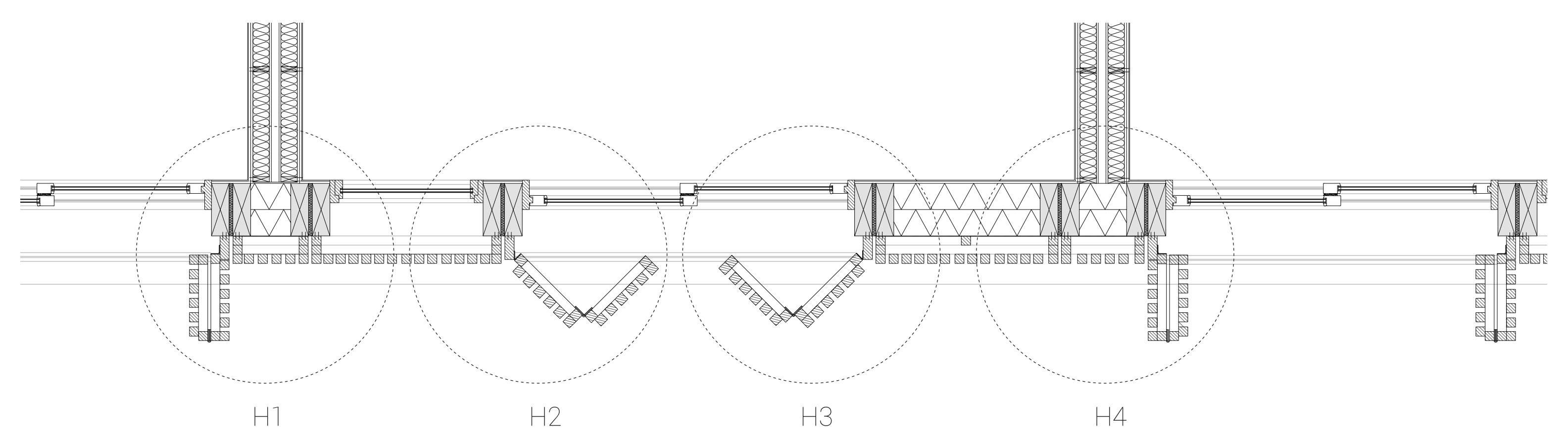
Horizontal section upper part 1:20
