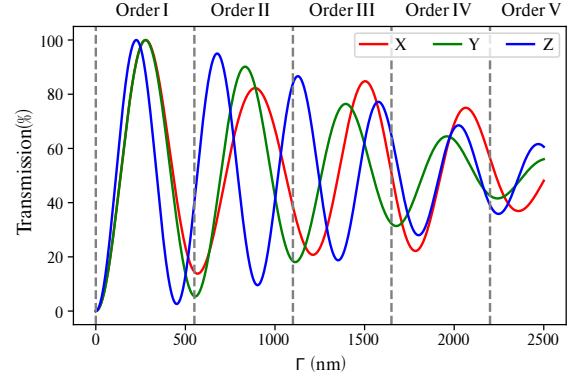
Figure 5: Theoretical color response of a liquid crystal.
