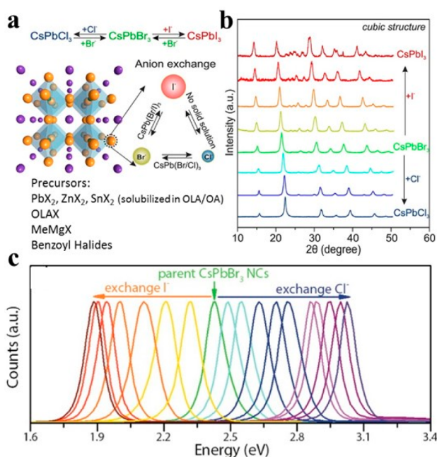
Figure 25. (a) Scheme of the AE reaction involving CsPbX 3 NCs. (b) XRD patterns and (c) PL spectra of CsPbX 3 (X = Br, Cl, or I) NCs prepared by AE from CsPbBr 3 NCs. Reproduced from ref 21. Copyright 2015 American Chemical Society.
