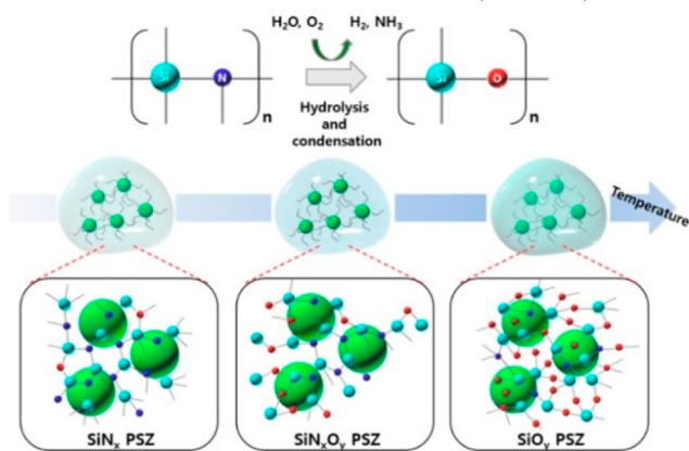
Scheme 15. Sol–Gel Route (Moisture-Induced Hydrolysis), Based On the Use of Liquid PSZ, Employed to Protect the Surface of LHP with Either SiN x , SiN x O y , or SiO y a
