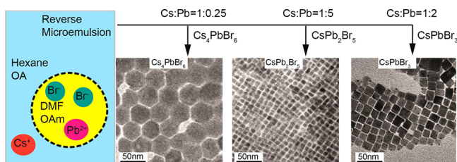
Figure 20. Illustration of the micelle structure that is formed in the reverse microemulsion process, which comprises an “oil” phase with n -hexane, and an “aqueous” phase with DMF. TEM images of Cs 4 PbBr 6 , CsPb 2 Br 5 , and CsPbBr 3 perovskite NCs formed with the different Cs:Pb:Br feed ratios. Reproduced from ref 222. Copyright 2017 American Chemical Society.
