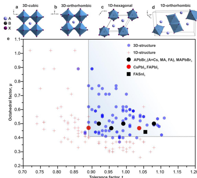
Figure 1. Schematic representations of (a) an ideal 3D cubic structure, as observed in \alpha\text{-FAPbI}_3 ; (b) an orthorhombically distorted 3D structure, typically reported for \text{CsPbBr}_3 ; (c) a one-dimensional (1D) hexagonal lattice, found in the yellow phase of \text{FAPbI}_3 ; and (d) a 1D orthorhombic structure, found in the yellow phase of \text{CsPbI}_3 . (e) Reported 3D and 1D structures of different all-inorganic and hybrid organic–inorganic \text{ABX}_3 MHP compounds. The light blue squared area represents the region in which stable compounds are located. The tolerance and octahedral factors were mainly taken from the report of Travis et al. 66 All panels are reproduced from ref 67. Copyright 2017 American Chemical Society.
