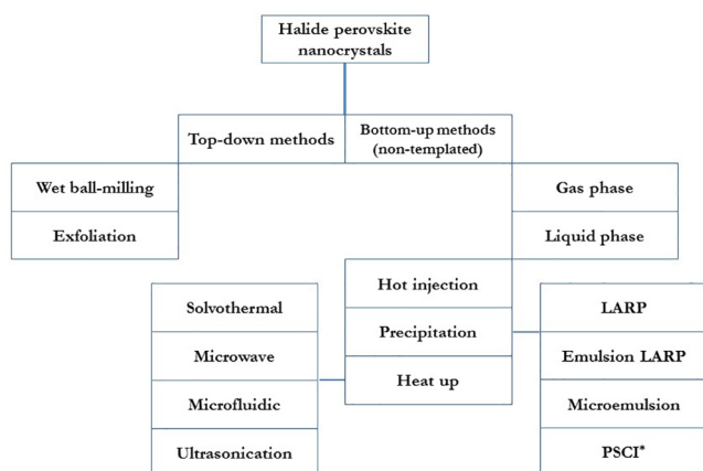
Scheme 1. Outline of the Various Methods Employed in the Synthesis of MHP Nanocrystals
