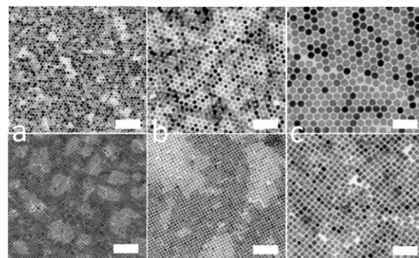
Figure 21. (a–c) TEM images of CsBr NCs of three representative sizes (top panels) and the resulting CsPbBr 3 NCs (bottom panels) that were obtained after the addition of Pb-oleate. Scale bars correspond to 50 nm in all panels. All panels are reproduced from ref 225. Copyright 2018 American Chemical Society.
