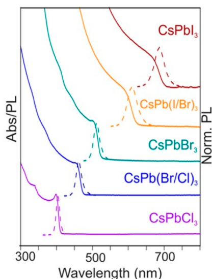
Figure 29. Bandgap tuning of \text{CsPbX}_3 NCs as a function of halide content, as demonstrated by UV-vis and PL spectra. Reproduced from ref 26. Copyright 2015 American Chemical Society.
