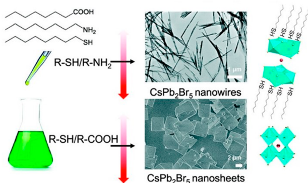
Figure 13. LARP synthesis of \text{CsPb}_2\text{Br}_5 NWs and NSs. Reproduced with permission from ref 201. Copyright 2017 American Chemical Society.
