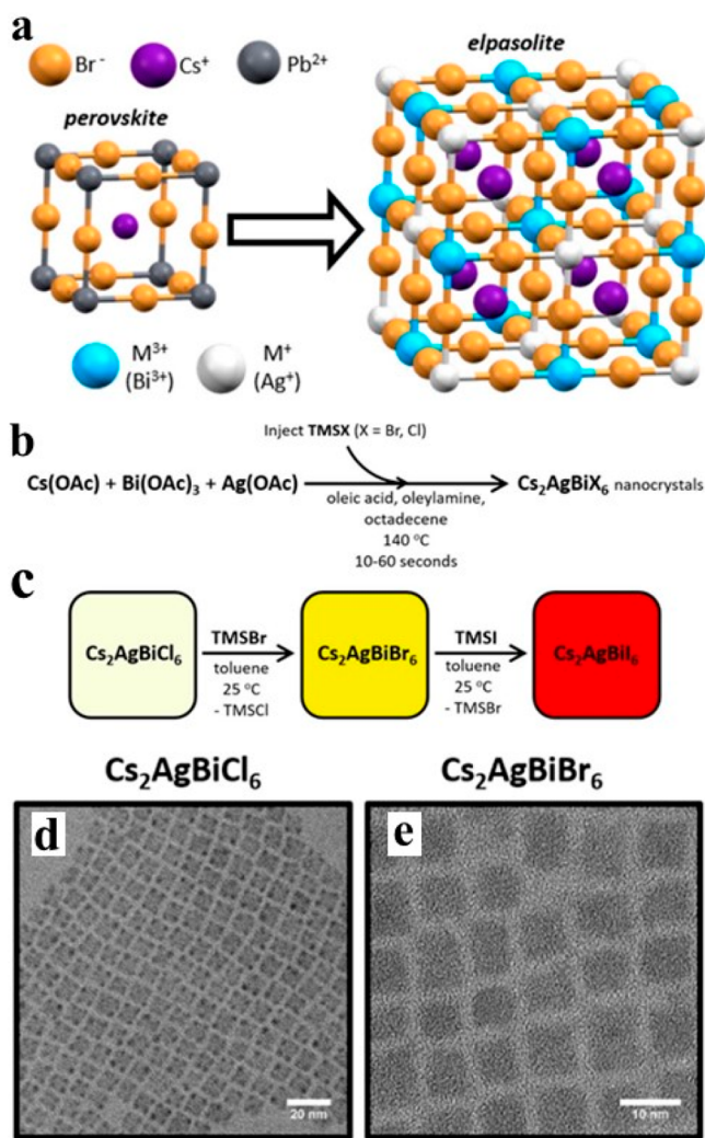
Figure 9. (a) The structure of a double perovskite crystal (e.g., \text{Cs}_2\text{AgBiBr}_6 ). (b) Scheme of the HI synthesis of \text{Cs}_2\text{AgBiX}_6 NCs and (c) their postsynthesis anion-exchange reactions using trimethylsilyl halide reagents. TEM images of (d) \text{Cs}_2\text{AgBiCl}_6 and (e) \text{Cs}_2\text{AgBiBr}_6 NCs. All panels are reproduced from ref 115. Copyright 2018 American Chemical Society.
