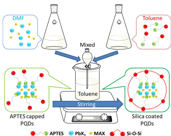
Scheme 14. Encapsulation of MAPbX 3 NCs in a Silica Matrix Using a LARP-Based Approach Together with Triethoxysilane (APTES) a
