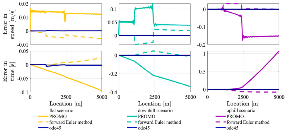
Fig. 7. Comparison of the error in speed (up) and time (down) at each location with respect to the analytical method for flat (left), downhill (middle) and uphill (right) slopes between 1100 and 2400 m. In each plot the dark blue line represents the error of MATLAB's ode45 function with respect to the analytical formulas, while the coloured dashed lines represent the error of the forward Euler method, and the coloured continuous line represent PROMO's error.
