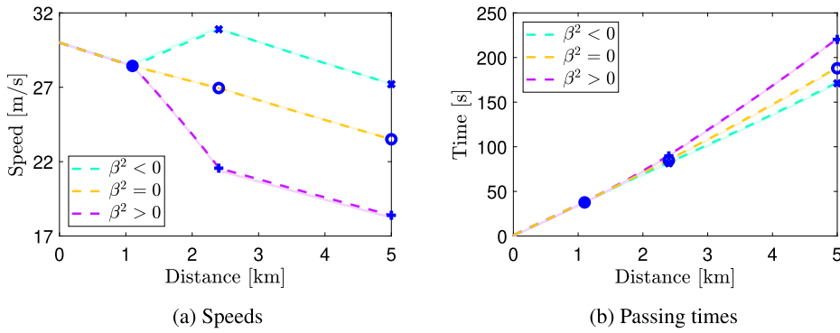
Fig. 6. Comparison of the coasting curves generated by the three methods.
