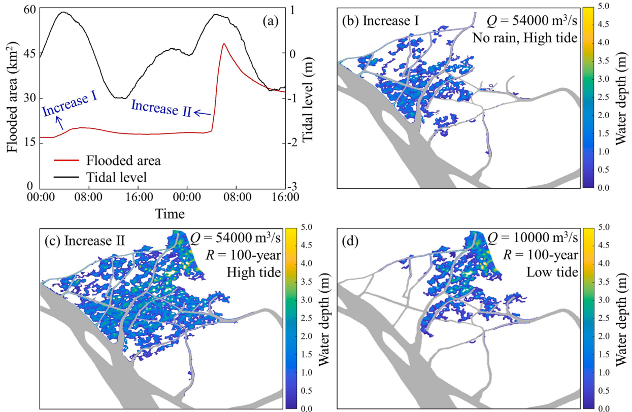
Fig. 11. (a) The time-varying curve of the flooded area for the most extreme compound flooding; The maximum flooded area for (b) Increase I, (c) Increase II, and (d) the rainfall dominated scenario.
