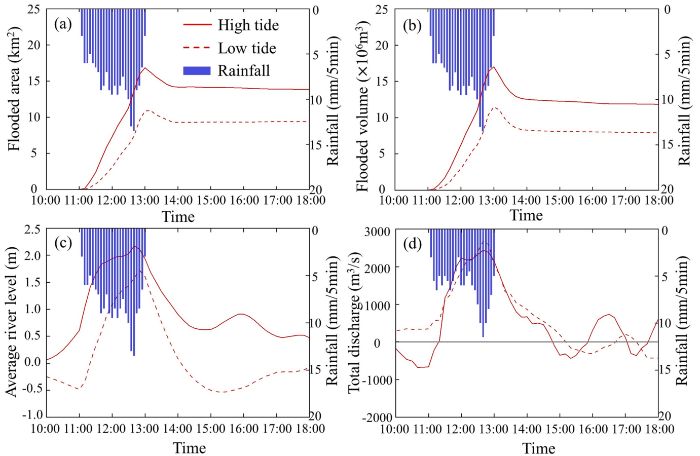
Fig. 8. Flooding process for low Modaomen flow under different astronomical tidal levels: (a) flooded area; (b) flooded volume; (c) mean water levels of the river network; (d) total river discharge of the river network.
