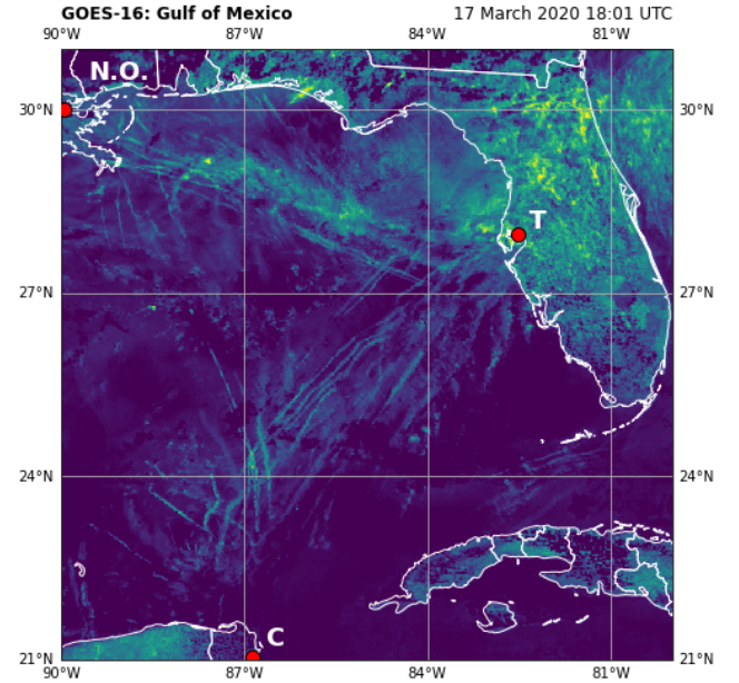
Figure 4. GOES-16 12.3-10.35 \mu m (BTD) image over the Gulf of Mexico, where contrails are visible of flights flying between i.a. New Orleans (N.O.), Tampa (T) and Cancún (C).
