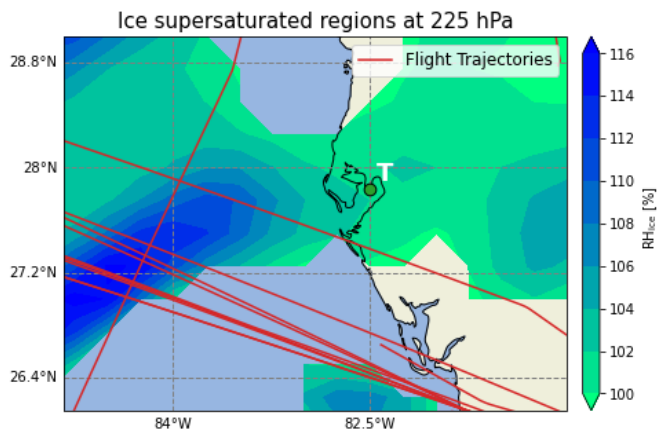
(a) ISSR for section of Florida, location of Tampa indicated by T (2020-03-18 18:00 UTC), with flight trajectories in red flying at cruise close to the ISSR.
