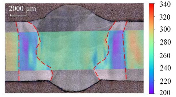
a) S700 weld zone
