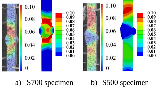
Figure 7 True strain contour plot in the unmilled welded coupon specimen
