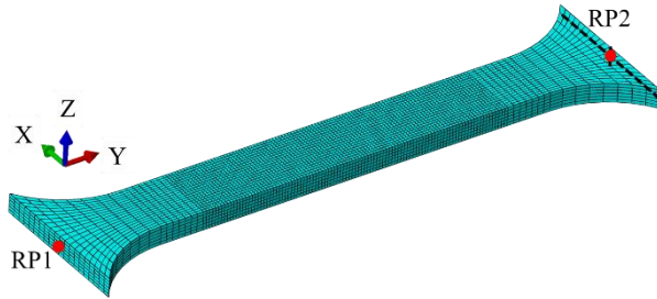
a) Milled welded coupon specimen
