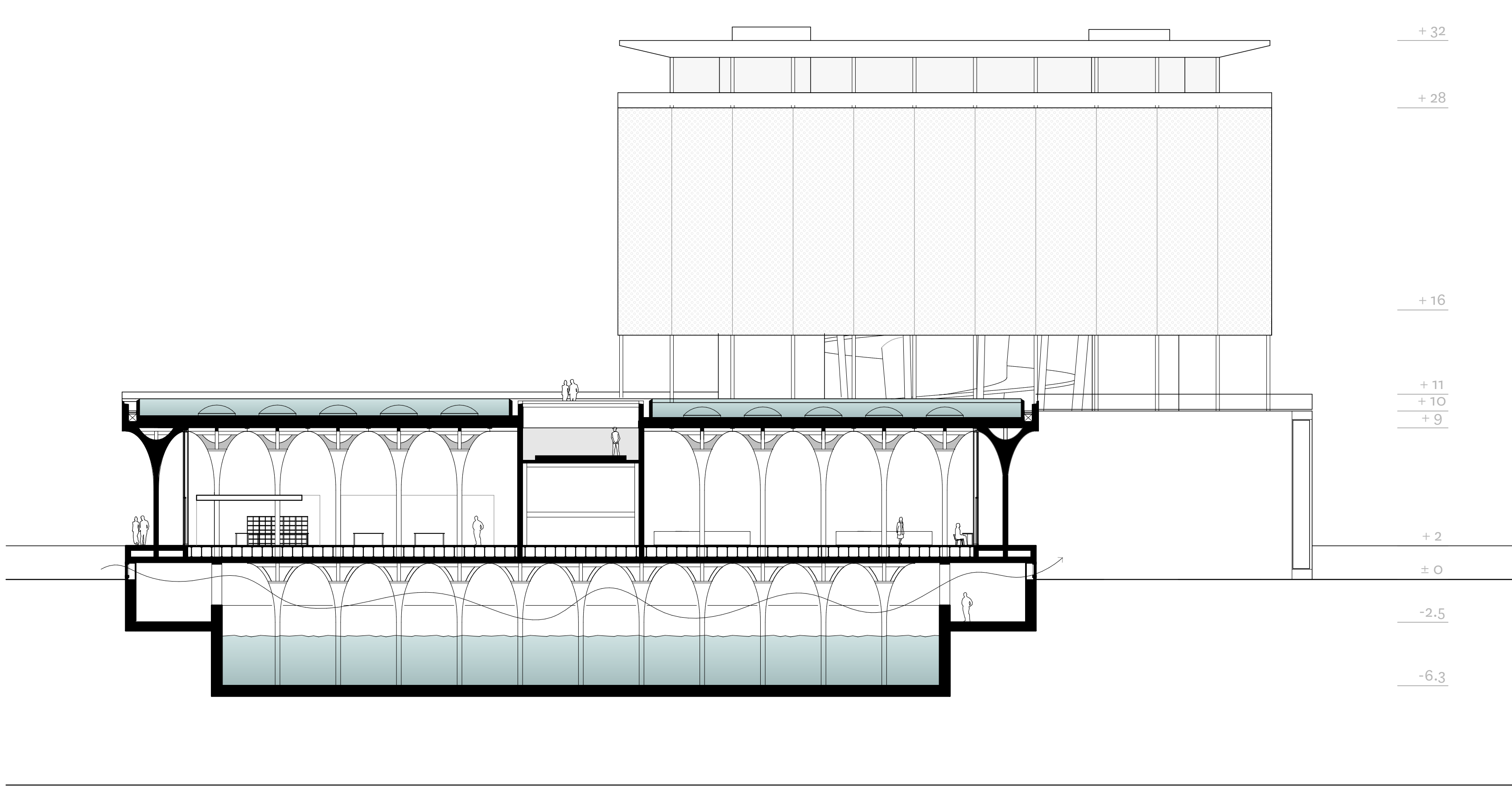
Cross section B-B 1:200
