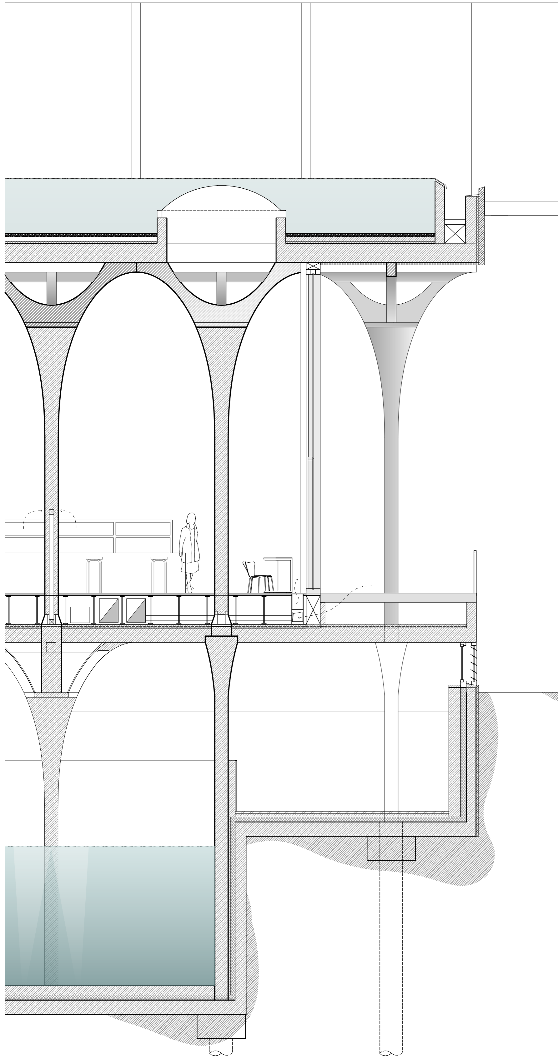
Section fragment D 1:50
