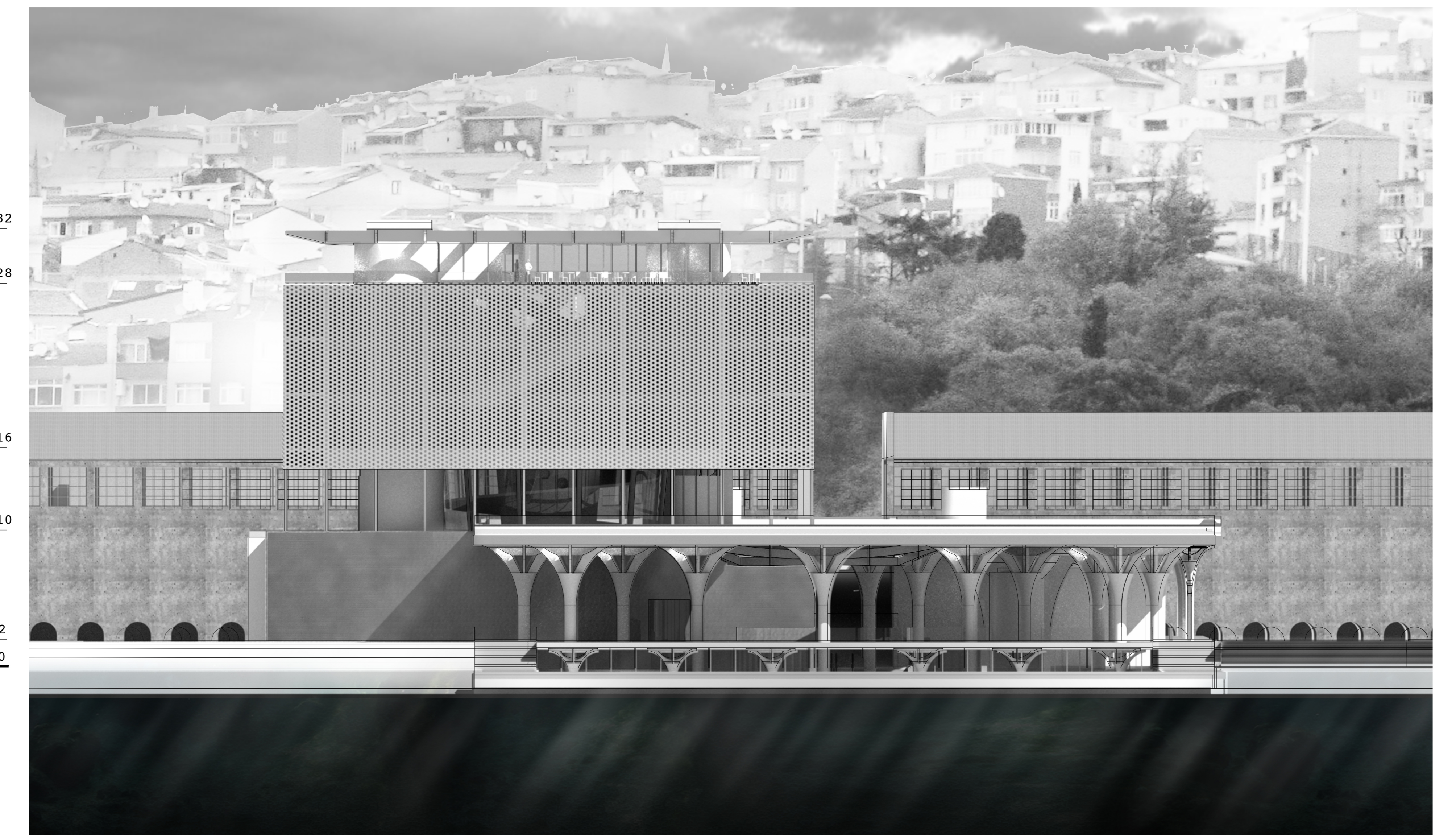
Elevation West 1:200
