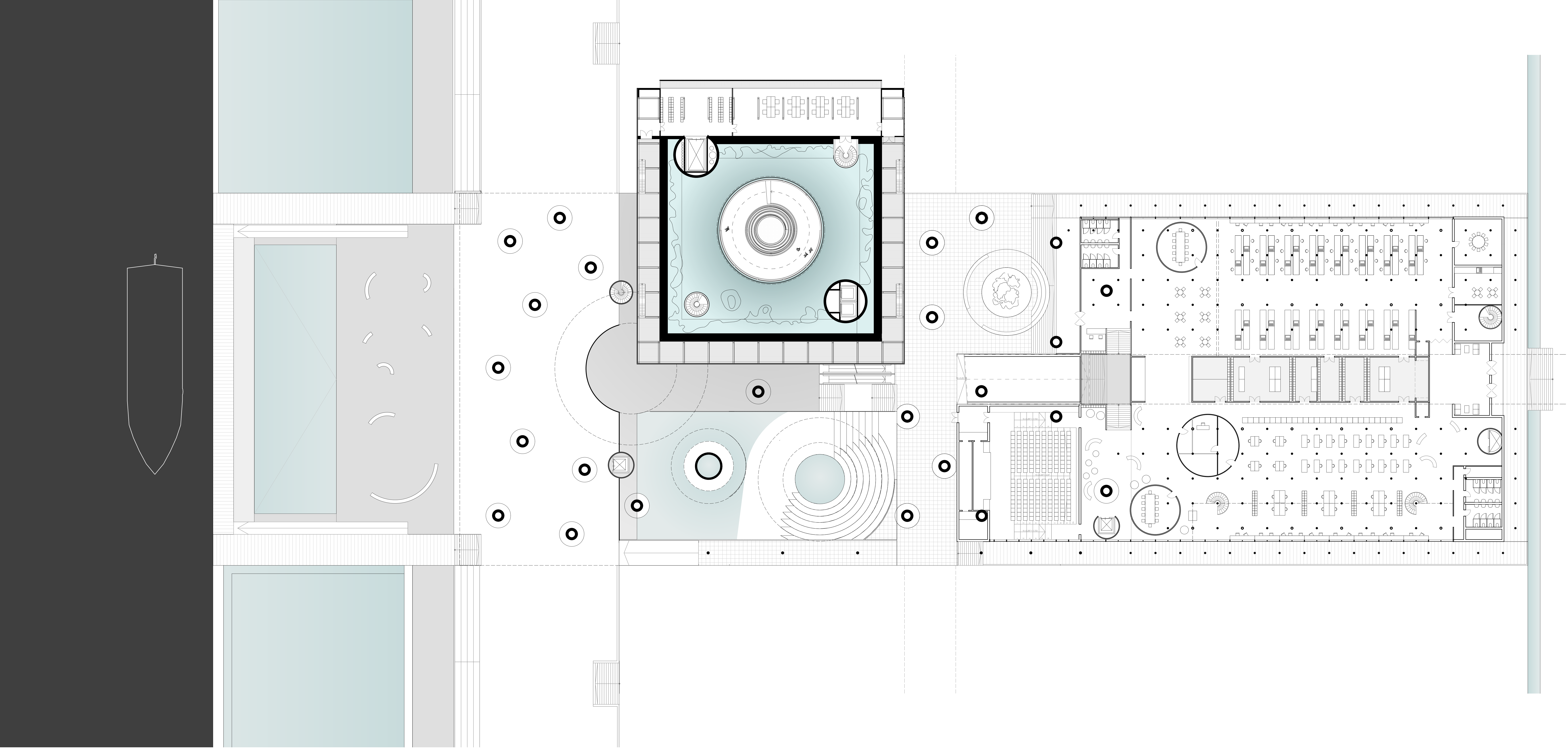
PLAN Level +2m 1:200
