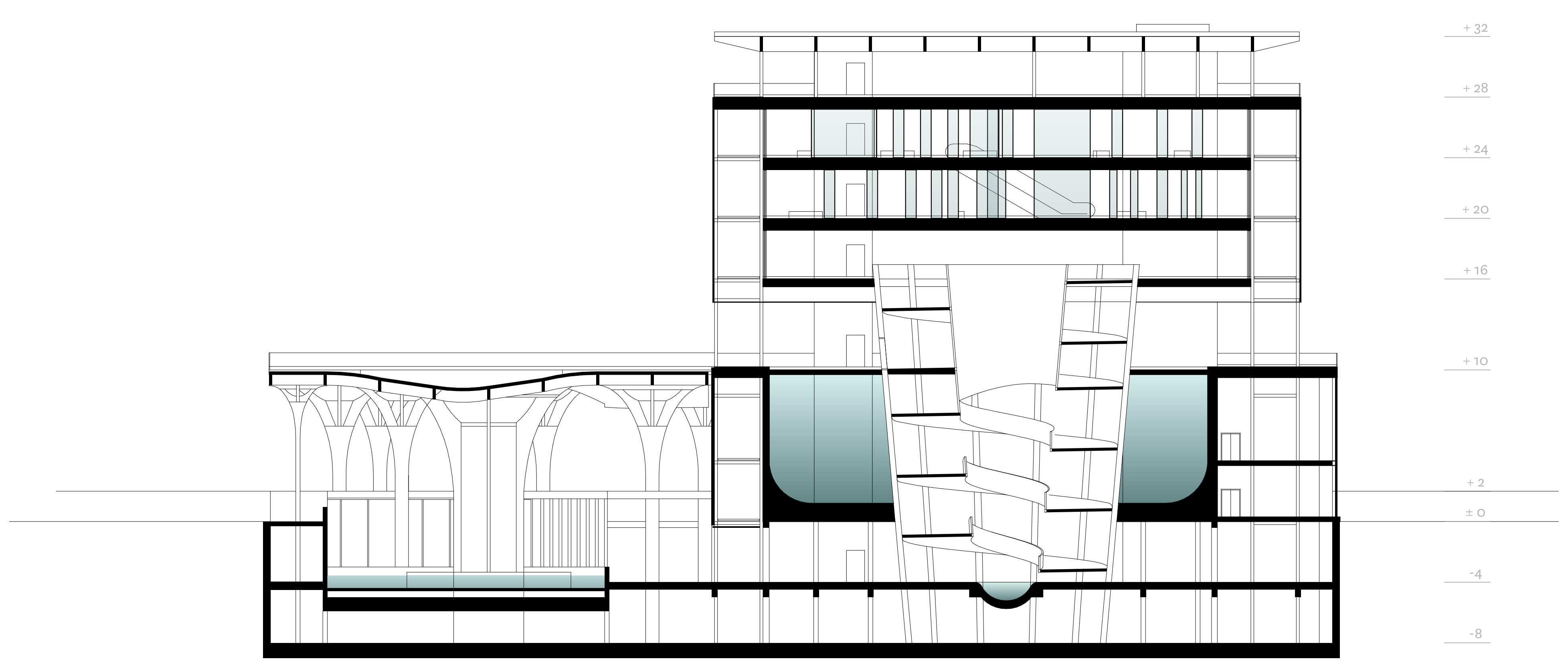
Cross section C-C 1:200
