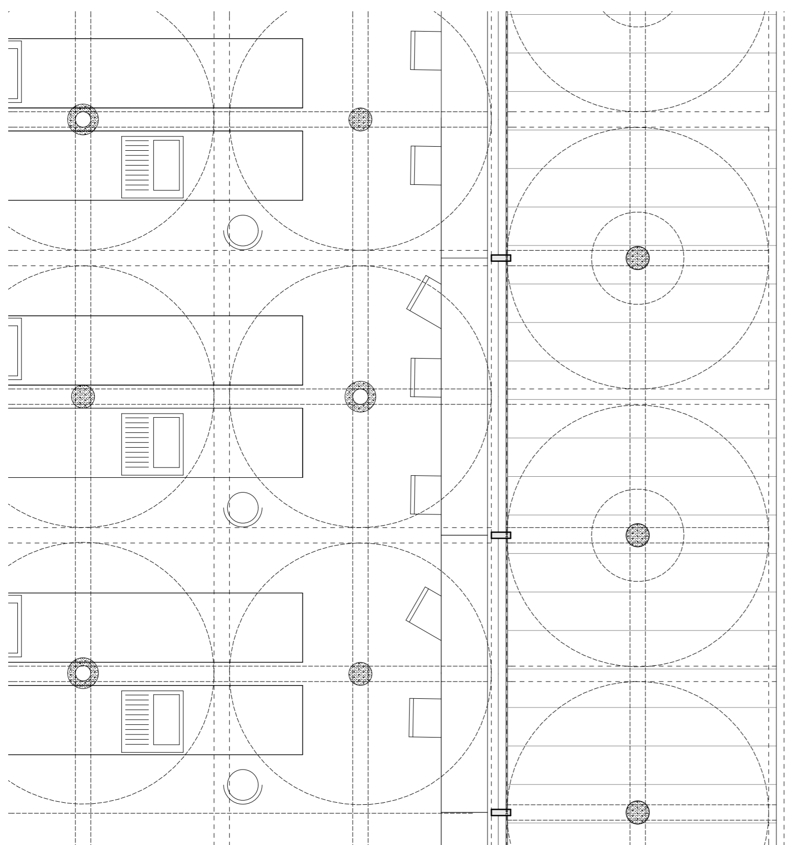
Horizontal cross-cut D 1:50
