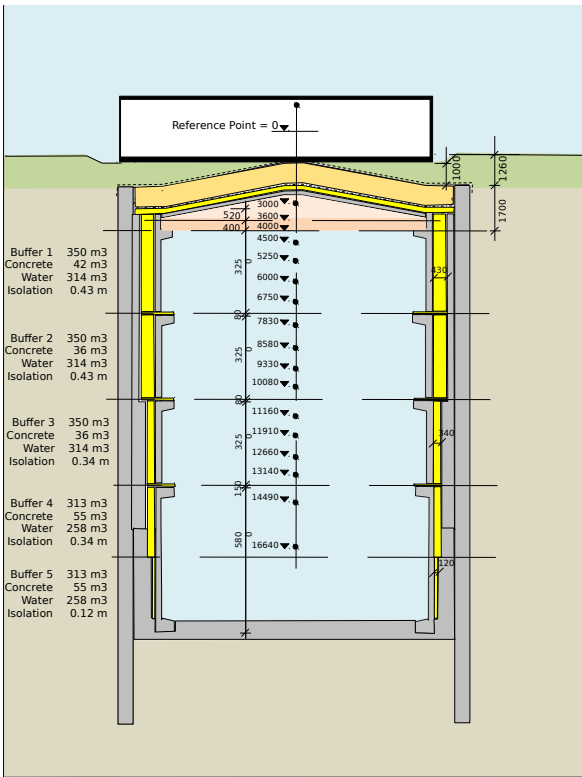
Figure 7.3: Technical schematic diagram of the Ecovt. All dimensions are given in mm (unless specified otherwise).
