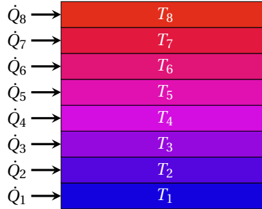
Figure 6.2: Example of the layout of the spatial discretization made by a 1D model. The tank is controlled by the external input heat \dot{Q}_i and the 1D model uses 8 layers. The colors represent the difference in temperature due to stratification.
