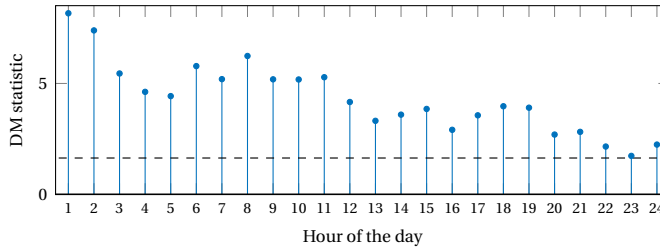
Figure 3.5: DM test results when comparing M_{\text{NoFR}} and M_{\text{FR}} . Values above the dashed line reject the null hypothesis with a 95% confidence level, and in turn, represent cases where the accuracy of M_{\text{FR}} is significantly better.
