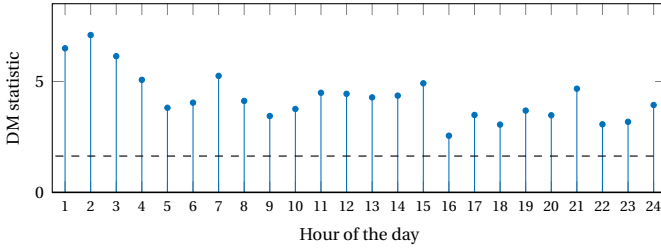
Figure 3.6: DM test results when comparing M_{\text{NoFR}, l_B} and M_{\text{FR}, l_B} . Values above the dashed line reject the null hypothesis at a 5% significance level, and in turn, represent cases where the accuracy of M_{\text{FR}, l_B} is significantly better.
