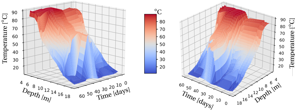
Figure 7.12: Optimal temperature evolution in the vessel over the 2-months period.
