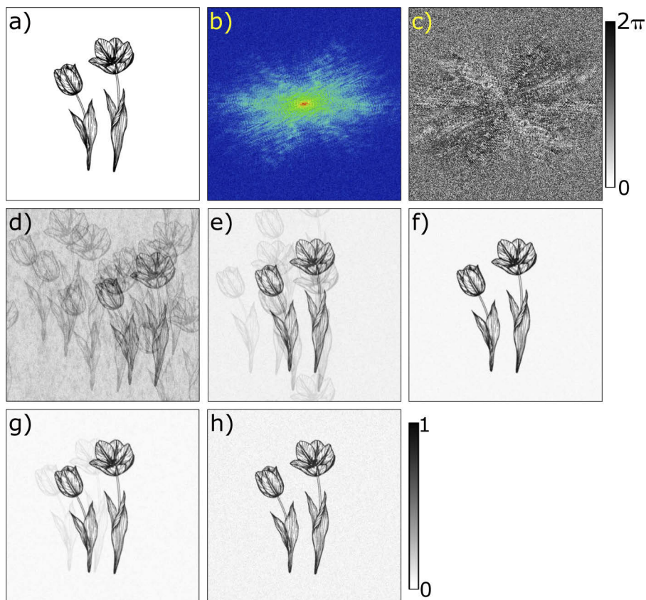
Fig. 2. Numerical simulations of the algorithm performance as a function of number of included measurement angles. (a) Intensity image of the simulated object (a flat phase is assumed) (b, c) Far-field DSI intensity (b) and phase (c) pattern as they would be recorded in an experiment. (d-g) Reconstructed images of the object when including data respectively from two, three, four and five measurements recorded at different angles. Each of these images is the average of 10 independent reconstructions. (h) Typical result for a single reconstruction, using diffraction signals at five different shear angles. The colorbar bar right of (h) applies to all intensity images of the object.
