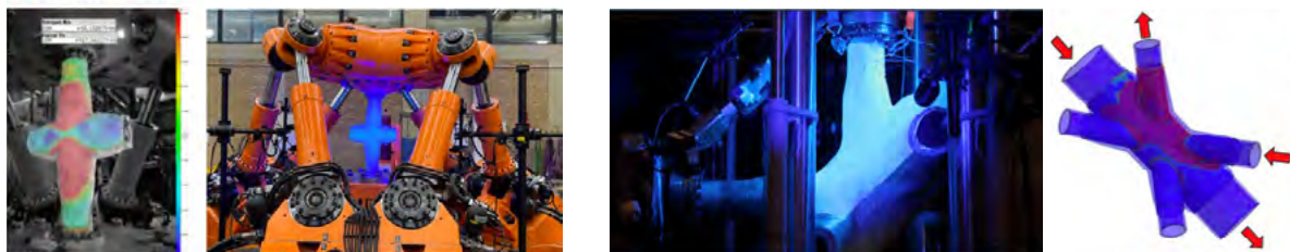
Figure 3. Multi-axial loading test in Hexapod (6 DOF test rig) and tests on KK joints (multi-planar).
