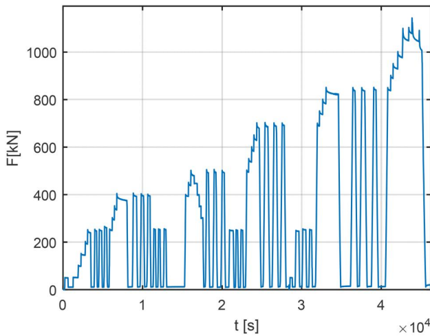
Figure 8. Loading protocol for SR3M1 (Zarate Garnica & Lantsoght, 2021).
