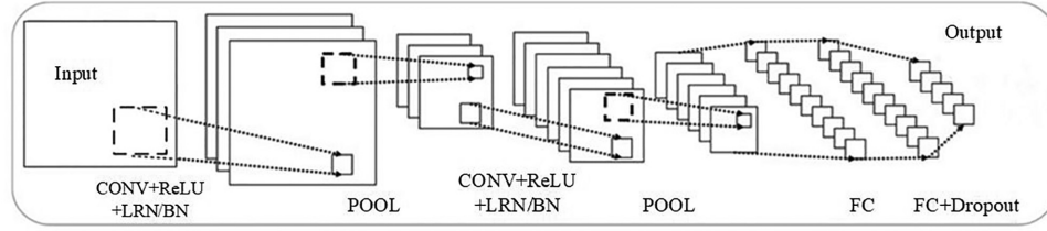
Figure 6. Illustration of a typical convolutional neural network.
