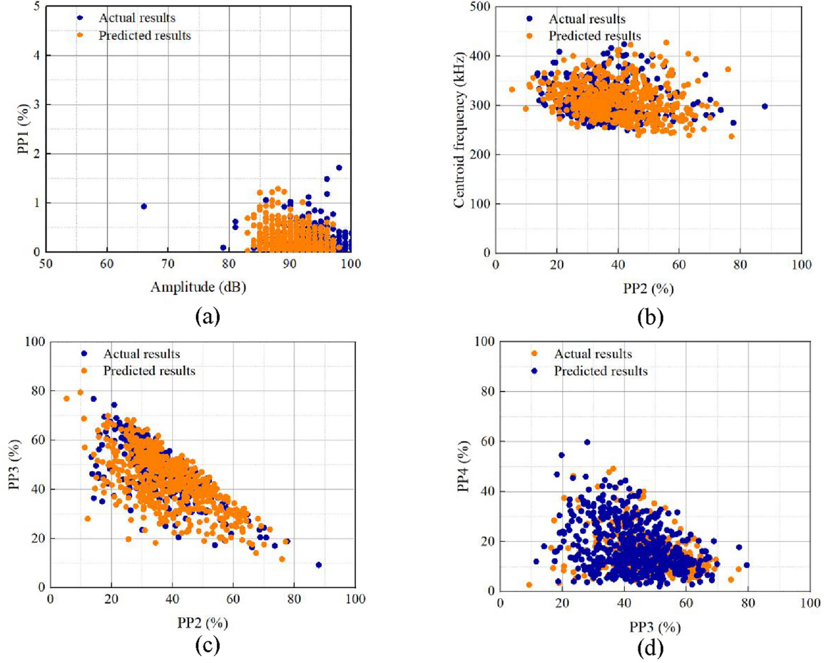
Figure 22. Distributions of AE parameters extracted from actual and predicted results.
