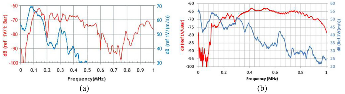
Figure 9. Frequency sensitivity spectrum of (a) R15α sensor, (b) WSα sensor.
