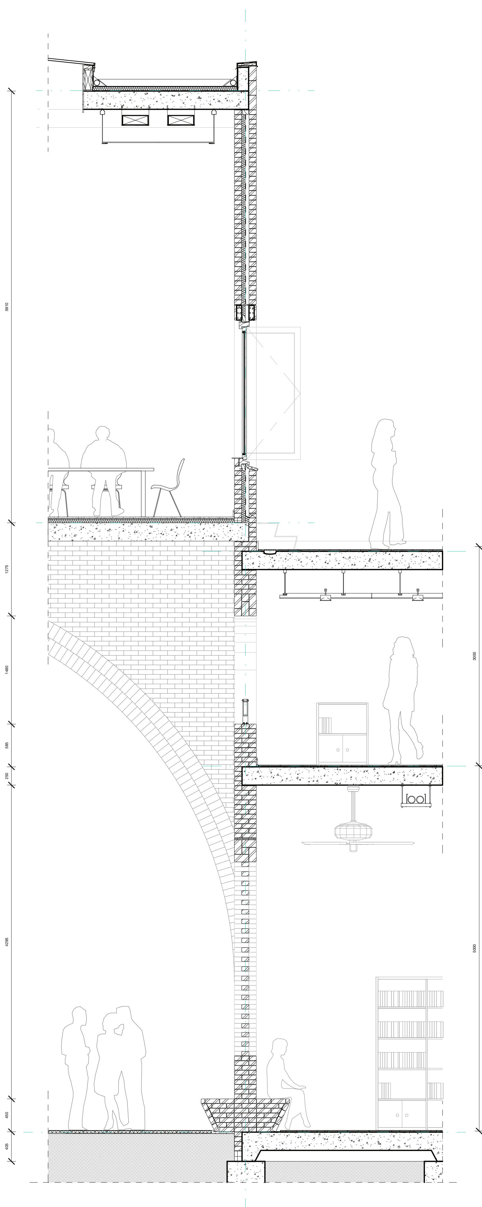
FACADE DETAIL
