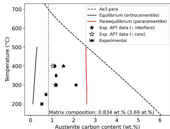
Fig. 10. Phase diagram with predicted austenite carbon compositions assuming the CCE model. Experimental data obtained from SXRD are shown as circles. The error bars are related to the standard deviation of carbon chemical content calculated using different austenite peaks. Filled and opened star symbols are the values obtained from APT measurements at the austenite interface and core, respectively. Black and red solid lines are expected austenite carbon content assuming equilibrium and paraequilibrium, respectively.
