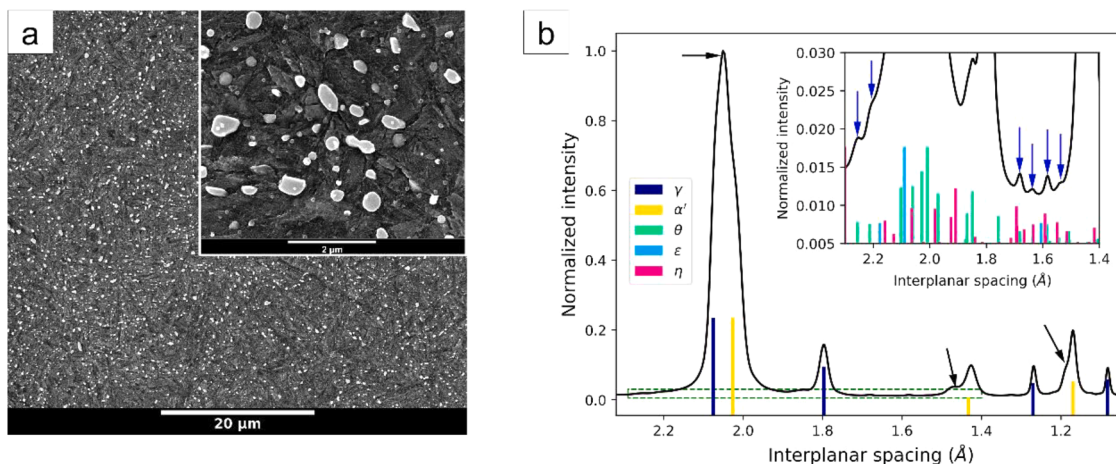
Fig. 2. (a) Scanning electron micrograph after cooling from 865 °C to room temperature. (b) High-resolution diffraction pattern of the initial condition. Black arrows indicate the splitting of martensite peaks, which occurs due to the high martensite tetragonality. Blue arrows indicate the peaks that cannot be indexed as either martensite or austenite, therefore being associated to carbides.
