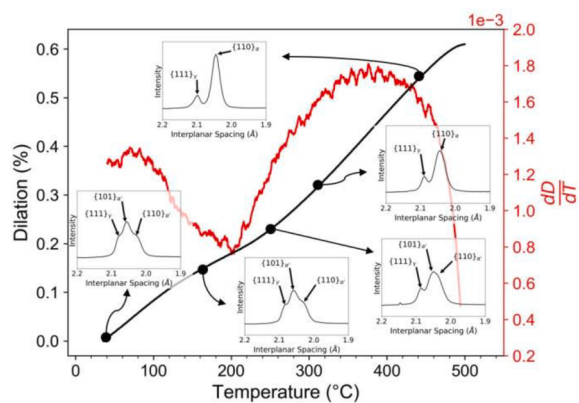
Fig. 3. Temperature vs. relative dilation during heating to the partitioning step showing the separation of the \{111\}\gamma , \{101\}\alpha' , and \{110\}\alpha' peaks with increasing temperature. The red curve shows the derivative of the dilation curve.
