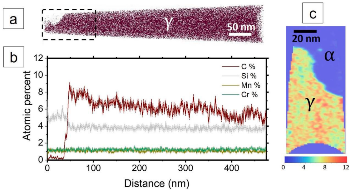
Fig. 7. Atom probe analysis obtained after tempering at 300 °C for 30 min showing: (a) Qualitative carbon map in the \alpha'/\gamma interface region; (b) Proxigram results for C, Si, Mn, and Cr along cylinder region A shown in (a); (c) Heat map for carbon content obtained from the selected area showed in (a). The scale bar shown in (c) is related to at.% in carbon.
