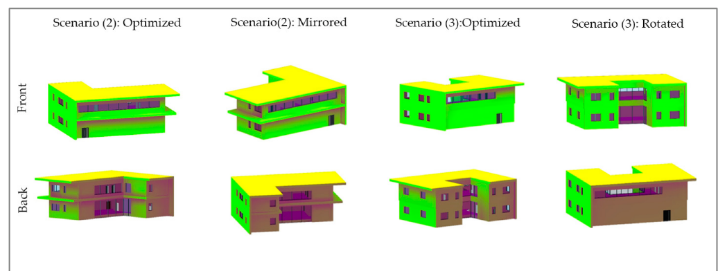
Figure 7. Comparison of orientation effects between the L-shaped and U-shaped scenarios Surface colors represent annual incident solar radiation (kWh/m 2 /year), where yellow–green indicates higher solar exposure and purple–brown indicates lower solar exposure.
