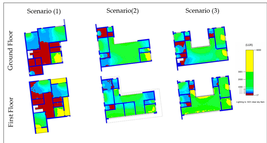
Figure 4. Comparison of daylight analysis results across the refined scenarios.
