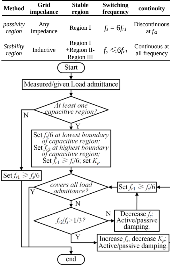
Fig. 11. Stability-oriented design of SAPF
