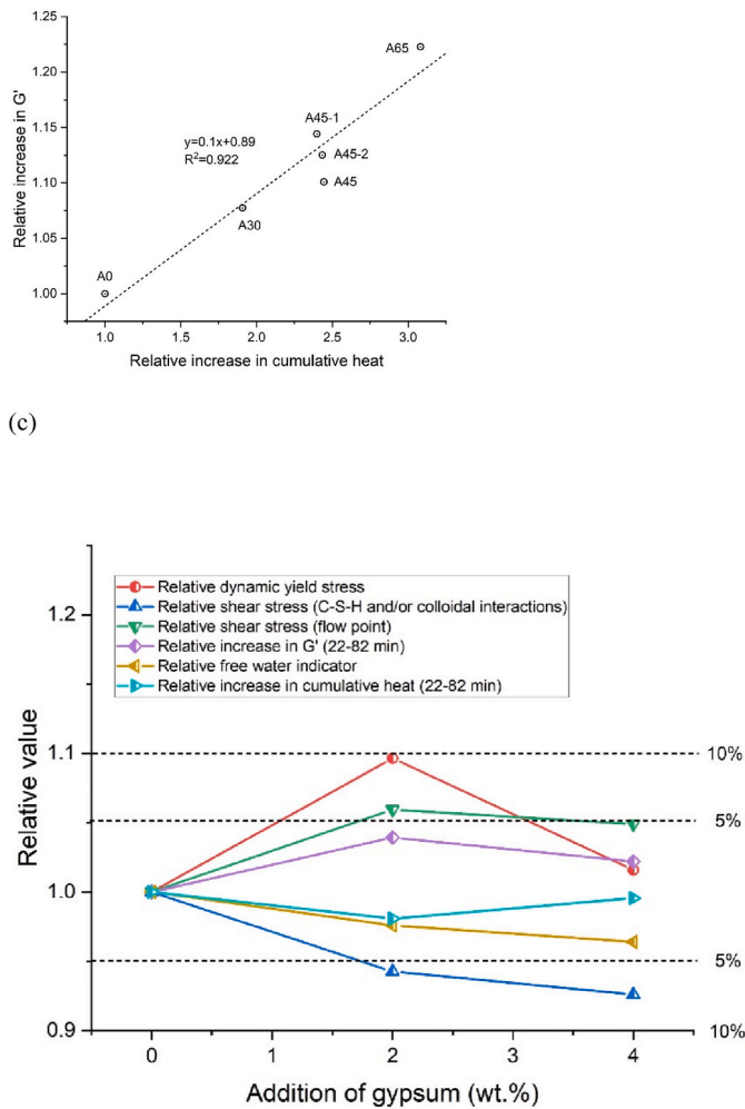
Fig. 18. Influence of increasing gypsum content on rheological characteristics, evolution of elasticity and rigidity (22–82 min), free water indicator and early-age hydration (22–82 min). All plotted values were relative to the value of mixture A45 (0 wt% gypsum). The dashed lines represent the relative change of 5% and 10%.
