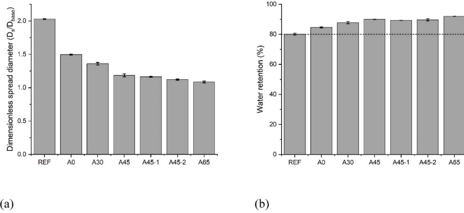
Fig. 5. (a) Mini-slump flow test results-dimensionless spread diameter of fresh mixture at 10 min; (b) Water retention test result (measured after 1 h). Error bars represent the standard deviation of repeated test results.
