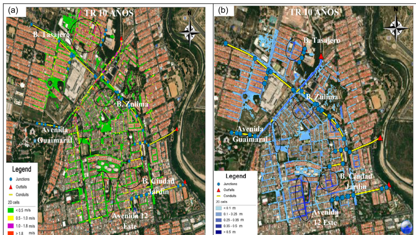
FIGURE 13 Hazard maps for Tr = 10 (a) velocity and (b) water depth.
