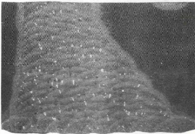
FIGURE 2.2. MACROSCOPIC EXAMINATION SPECIMENS SHOWING INCREASED POROSITY WITH DEPTH.
