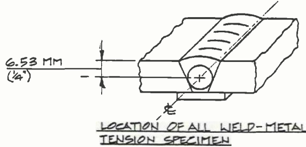
TEST PLATE SHOWING LOCATION OF TEST SPECIMENS
