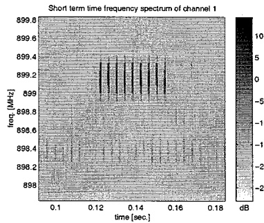
Fig. 2. Time-frequency spectrum of channel 1, showing GSM interference.
