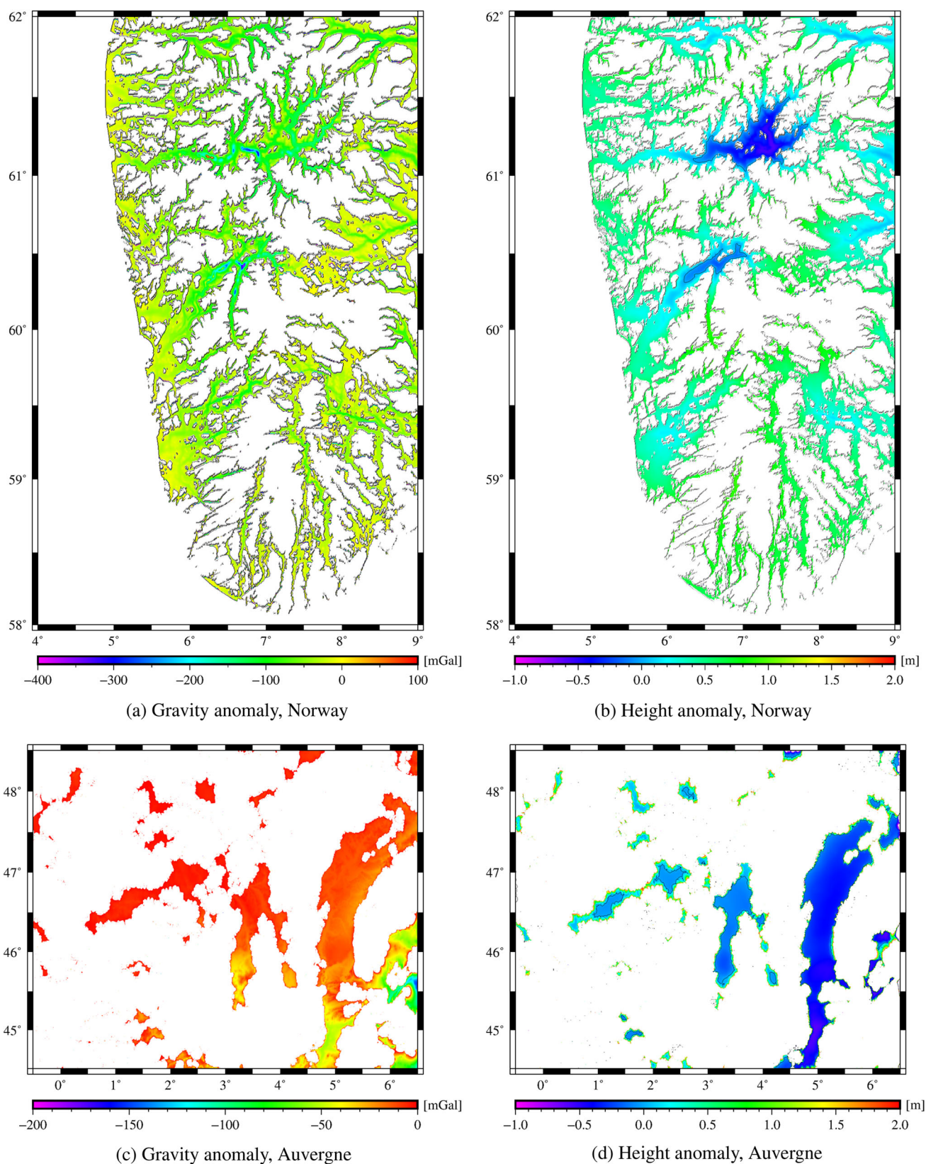
Fig. 3 Complete RTM correction to gravity anomaly and height anomaly in the Norway and Auvergne test areas. Shown are only the evaluation points which are located below the RTM surface
