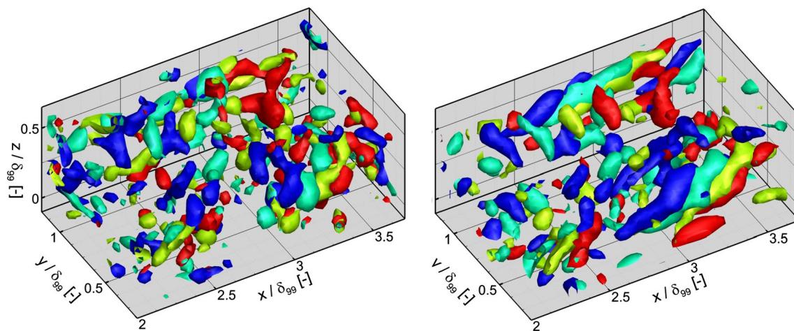
Fig. 12 Overview of coherent structures identified by the Q-criterion for MART N_M = 5 (left) and SMTE N_M = 5 (right). Regions A and B designate two convecting hairpin structures
