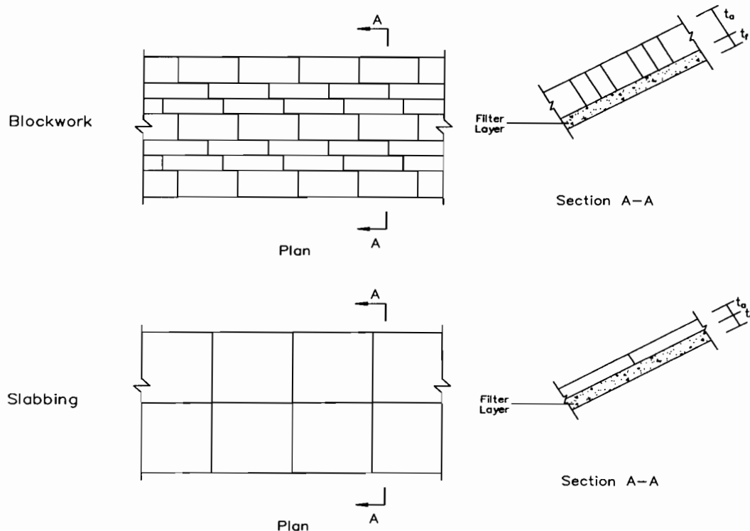
Figure 4.1 Typical blockwork and slabbing details
