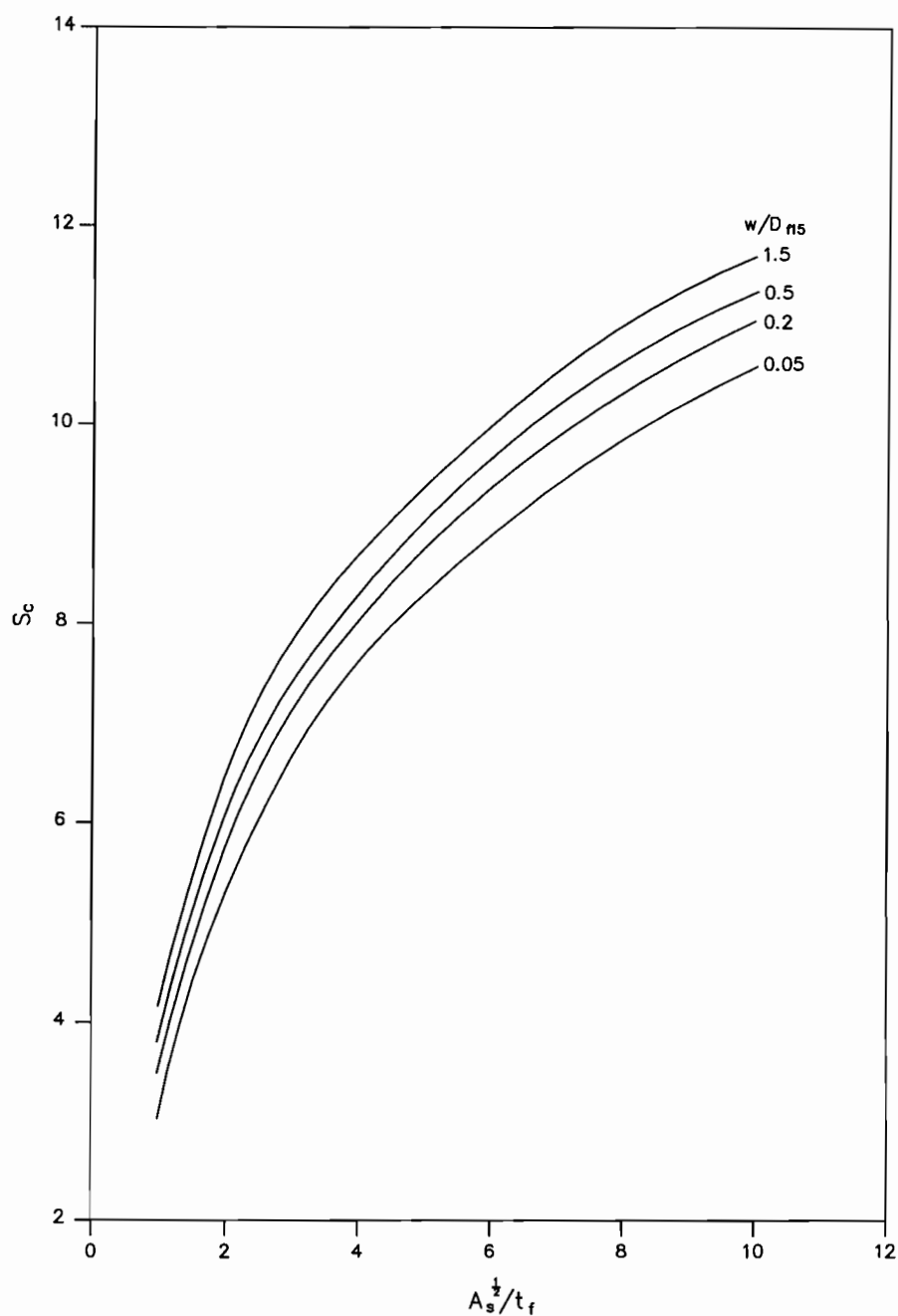
Figure 4.3 Design chart for slabbing
