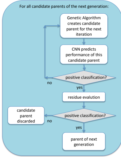
Figure 3: Flow-chart for the module ‘update acquisition geometry’ module with the convolutionan neural network, see Figure 2.
