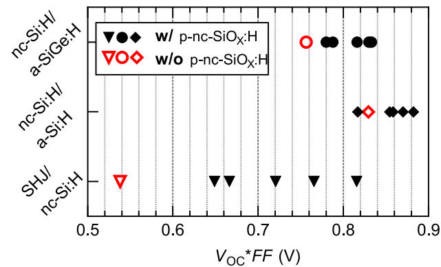
Fig. 8. V oc *FF product for 3 different tandem device architectures. Red icons indicate a single p-nc-Si:H layer in the TRJ. Black icons indicate 5 different bi-layer p-nc-SiO x :H/p-nc-SiO x :H + and p-nc-SiO x :H/p-nc-Si:H bi-layer configurations.
