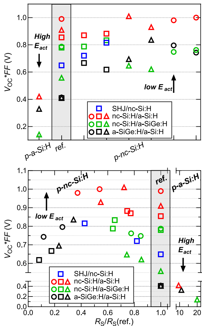
Fig. 6. The V_{oc} - FF product plotted as a function of the different contact layers (Top) and V_{oc} - FF product plotted as a function of change in series resistance ( R_s ) with respect to the reference sample without contact layer (bottom). Contact layers are processed on top of a 15–20 nm p-nc-SiO x :H layer. Tick marks in top plot indicate samples with a 5 nm p-a-Si:H contact layer, no contact layer (ref) and 6 different low E_{act} 3–6 nm p-nc-Si:H contact layers, processed at different conditions (gas flow rates, power). The arrows and E_{act} designation indicate the E_{act} in reference to that of the single p-nc-SiO x :H layer. The icons (triangle-square-circle) indicate series of samples processed at the same point in time with the exact same deposition conditions for all supporting layers. The colours indicates the multijunction architecture, namely SHJ/nc-Si:H (blue), nc-Si:H/a-Si:H (red), nc-Si:H/a-SiGe:H (green) and a-SiGe:H/a-Si:H (black).
