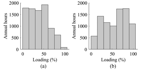
FIGURE 8. Yearly power demand for annual average loading ( P_{ave} ) of (a) 38% and (b) 57% [33].
