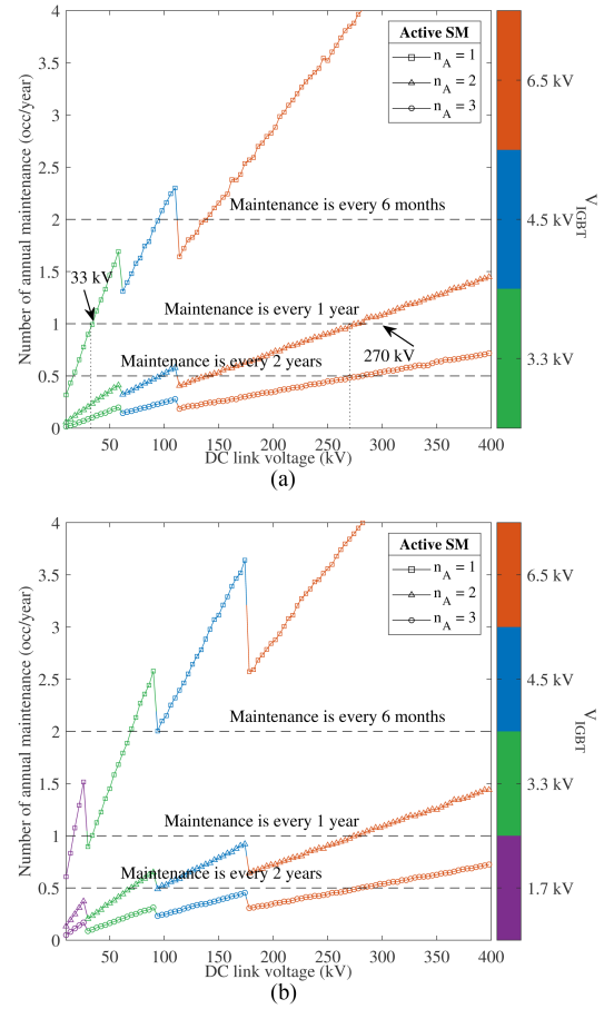
FIGURE 15. MCS results (10 000 trials) for estimating the number of maintenance frequency in the period of B_{10} = 10 years as a function of dc-link voltage at (a) 100% loading and (b) 38% loading.
