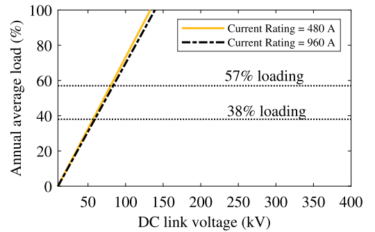
FIGURE 12. Sensitivity of the obtained results for feasibility boundary for the SRS and the MRS with higher rating switches.
