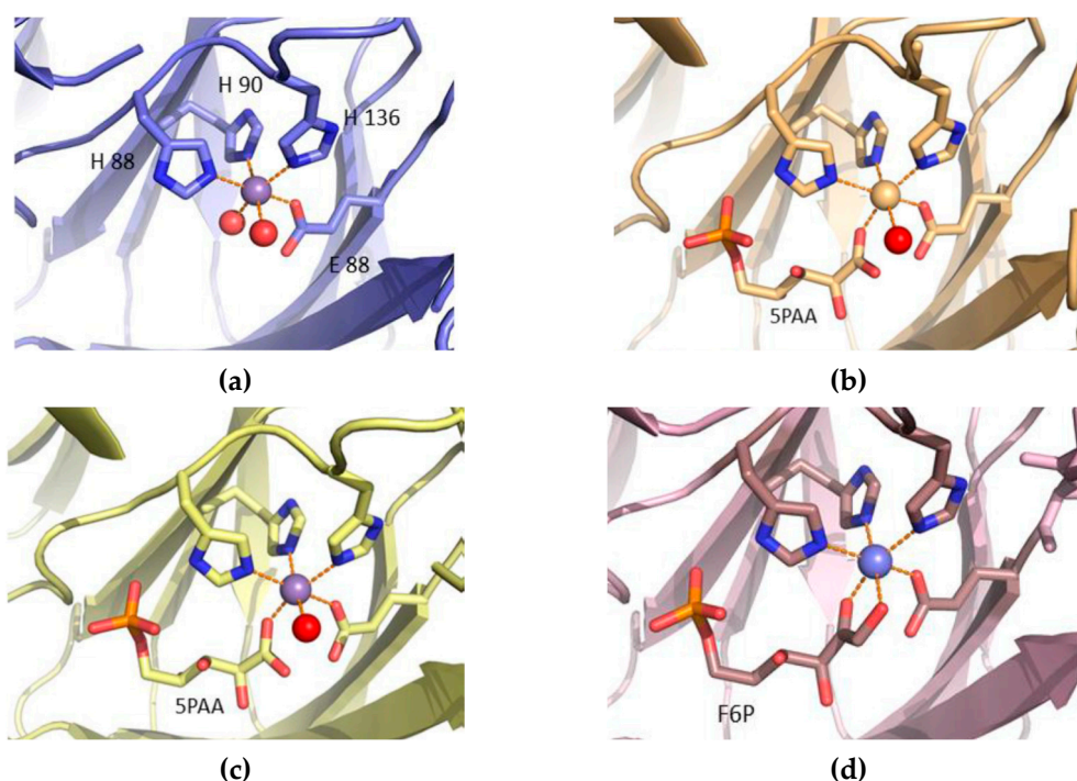
Figure 6. Mn^{2+} coordination in the mutant PfPGI structures. For all mutant structures, the Mn^{2+} ion (purple sphere) is coordinated in an octahedral arrangement: (a) Mutant AD (blue), (PDB code: 4LUL); (b) mutant RG (wheat), RG (PDB code: 4LTA); (c) mutant AG (yellow), (PDB code: 4LUK); and (d) mutant VY (pink), (PDB code: 4LUM), respectively. 5PAA and F6P shown as sticks.
