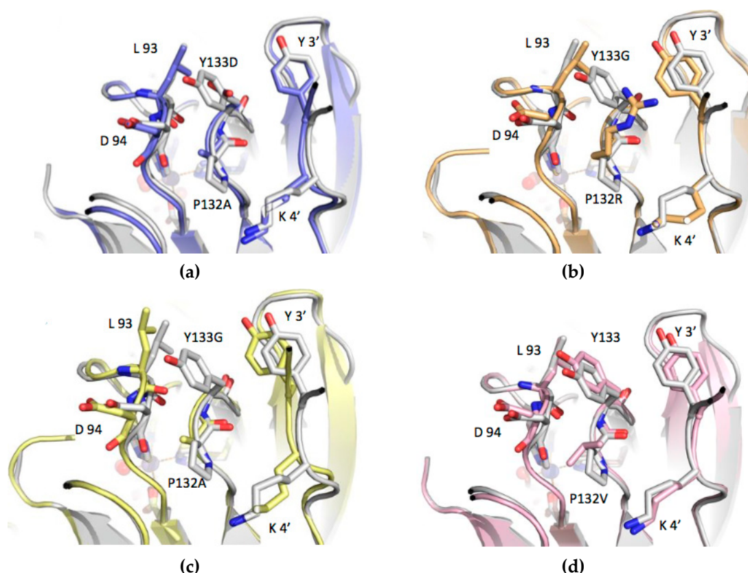
Figure 4. Comparison of the structure of the loops adjacent to the mutation position in the four mutant structures. In each panel, the structure of the wild-type enzyme (PDB code: 1X7N) is shown in white, with the relevant residues highlighted in stick representation and labelled. Y3' and K4' refer to the N-terminal strand from the adjacent subunit in the dimer. (a) Mutant AD (slate), (PDB code: 4LUL); (b) mutant RG (wheat), (PDB code: 4LTA); (c) mutant AG (yellow), (PDB code: 4LUK); and (d) mutant VY (pink), (PDB code: 4LUM).
