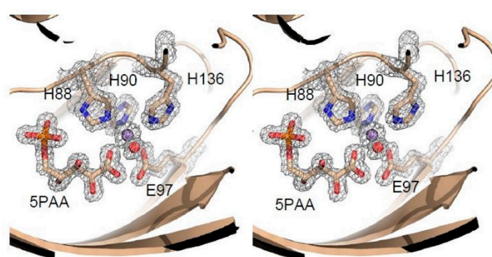
Figure 5. A stereo representation of the mFO–DFC electron density (grey mesh), contoured at 1.5 \sigma , for the P132A, Y133G mutant PfPGI structure (mutant AG, PDB code: 4LUK), showing the manganese (purple sphere), coordinating water (red sphere), 5PAA and metal coordinating residues (sticks).
