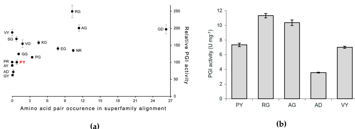
Figure 3. The results of activity measurement: (a) Graphical representation of the relative activity of each PfPGI mutant (Y-axis) compared to the amino acid pair occurrence according to the Cumulator-based CMA predictions (X-axis). All phosphoglucose isomerase (PGI) activities are relative to wild-type P. furiosus PGI (PfPGI; PY; in red). (b) The specific activity of wild-type PfPGI (PY) compared to selected high-occurrence/activity mutants P132R/Y133G (RG) and P132A/Y133G (AG), and lower or similar occurrence/activity mutants P132A/Y133D (AD) and P132V (VY). Manganese was used as co-factor and added via titration.
