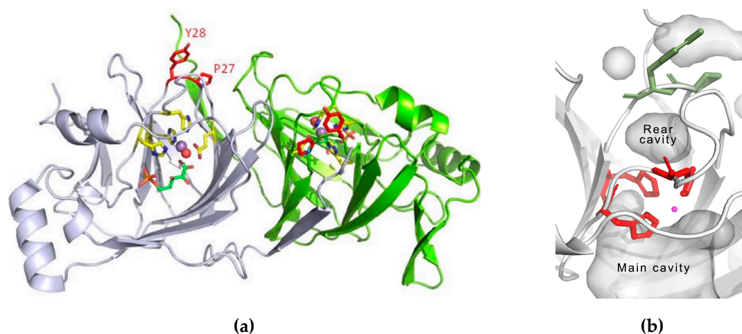
Figure 2. Structure details of wild-type PfpGI. (a) Cartoon representation of the dimer (white and green subunits) of the wild-type PfpGI Mn^{2+}/5PAA 3D structure (Protein Data Bank (PDB) code: 1X7N). The correlated amino acid pair “PY” is indicated in red. Shown in yellow are those residues involved in manganese (purple sphere) binding, including a water molecule (red sphere). The inhibitor 5-phospho-D-arabinonate (5PAA) is shown as a stick model (green). (b) Location of main and rear cavities in PfpGI structure. Histidines 88, 90, and 136 separating main and rear cavities are shown as red sticks, Pro132 and Tyr133 separating rear-side cavity from solvent as green sticks, Mn^{2+} ion as magenta.
