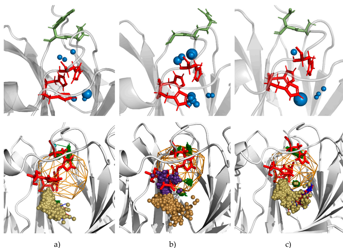
Figure 7. Pictures of water distribution (upper row) and water trajectories (lower row) in the vicinity of the Mn ion in molecular dynamics (MD) simulations of: (a) WT chain A (no or small movement of His88, observed in all variants representative for variants with similar to WT activity); (b) RG mutant chain B (with His88 rotation observed in chain B of mutants with higher activity), and (c) AD chain A (no rotation of His88, lowest water density, observed in mutant with lowest activity). Pictures were generated with PyMOL software based on AQUA-DUCT results. The water distribution pictures present water hot spots as blue spheres with size proportional to the local density of water molecules. Protein backbone—grey cartoon representation; His 88, 90, 136—red stick representation; residues 132 and 133—green stick representation; object—orange mesh; inlets—small balls. Green lines depict trajectories of trapped water molecules. Inlets colors: gold—main cavity cluster, violet—cluster observed due to His88 rotation, cyan—rear-side cavity cluster.
