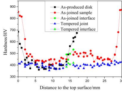
Fig. 4. Microhardness of the cross-sections of the as-produced disk and joined samples.
